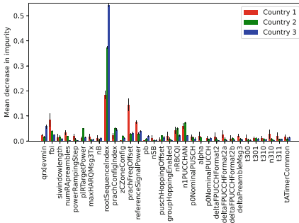
Fig. 4. Feature importance for the Random Forest model in our two inference scenarios. The variance reported refers to the results obtained over the different nested cross-fold runs.
