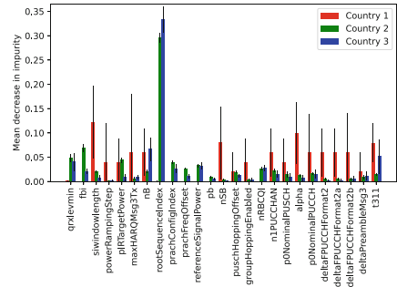
Fig. 4. Feature importance for the Random Forest model in our two inference scenarios. The variance reported refers to the results obtained over the different nested cross-fold runs.
