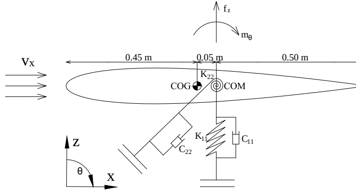
Figure 1: A two-degree of freedom model for the pitching and plunging motions of a prismatic wing.
