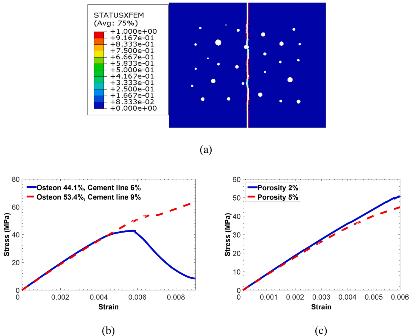
Fig. 9. (a) Crack propagation path in the four-phase model with a decrease in the percentage of osteon to the value of 44.1%; (b) the comparison of stress–strain diagrams of four-phase composite microstructure with different osteon percentage and cement line under tension; and (c) the effect of porosity (areal fraction of pores) on the stress–strain behavior of the bone microstructure.
