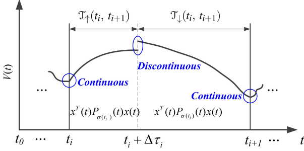
Fig. 2. The proposed Lyapunov function (6).
