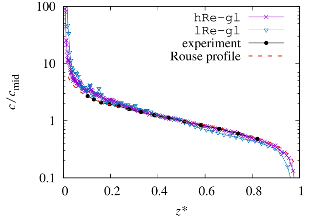
Fig. 11. Comparison: particle-concentration profiles from the simulations with lift force, and from experiments by Breugem and Uijttewaai (2006) and Breugem (2012). The particle-concentration profiles c are scaled by their respective particle-concentration in the centre of the channel c_{mid} = c(H/2) . The horizontal axis represents the wall-normal direction z which is scaled by the channel height H , denoted by z^* .
