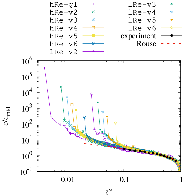
Fig. 22. Particle-concentration profile with closer look in the near-wall region.
