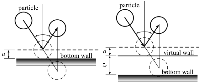
Fig. 3. The elastic bouncing wall for the particles: (left) bottom wall without virtual wall, (right) with virtual wall. a : particle radius, z_r : distance between virtual wall and bottom wall. The particles are relocated into a symmetrical position with reflective velocity.
