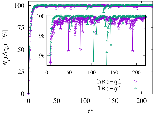
Fig. 10. Cases hRe-gl and lRe-gl: percentage of particles in the bottom layer \Delta z_b along the simulation time.
