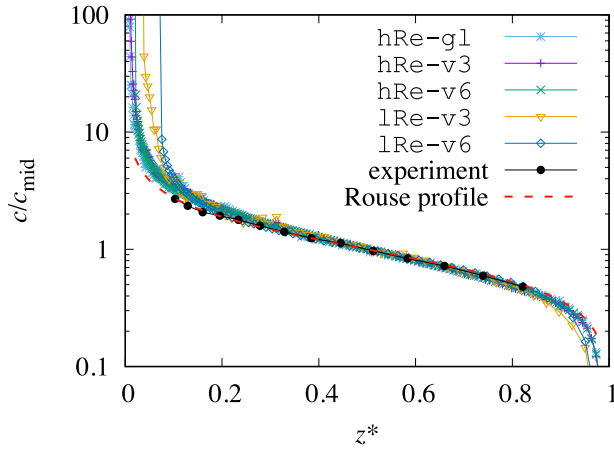
Fig. 14. Comparison: particle-concentration profiles from the simulations with virtual wall, and from experiments of Breugem and Uijttewaal (2006) and Breugem (2012). The particle-concentration profiles c are scaled by their respective particle-concentration in the centre of the channel c_{\text{mid}} = c(H/2) . The horizontal axis represents the wall-normal direction z which is scaled by the channel height H , denoted by z^* .
