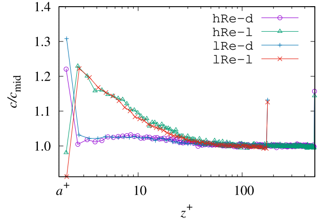
Fig. 6. Cases without gravitational force: particle concentration profile scaled by its value at z = H/2 (the middle of the channel). c_{\text{mid}} = c(z = H/2) .
