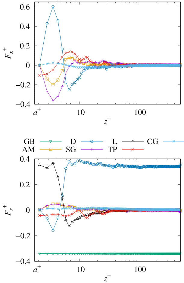
Fig. 12. Case hRe-g1: particle momentum profiles for Re_\tau = 500 , in wall-units: streamwise (up), wall-normal direction (down). GB: gravitational force, L: lift force, D: drag force, SG: stress-gradient force, AM: added mass force, CG: diffusion effect, TP: turbophoretic effect, L: lift force.
