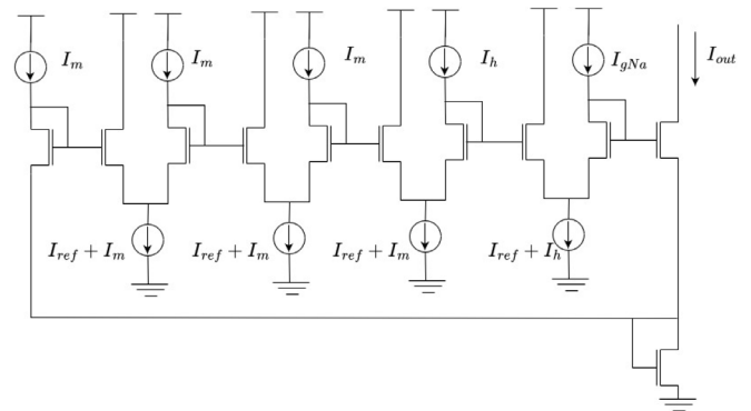
Fig. 8. Translinear circuit implementing a gated conductance of the form x^3y used to implement H-H conductance equations.
