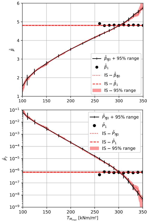
Figure 8. Verification of two-stage metamodeling approach for 10-variable problem against importance sampling solution, in terms of estimated reliability index \hat{\beta} and estimated probability of failure \hat{P}_f . Vertical line markers indicate the 95% confidence range of the results.
