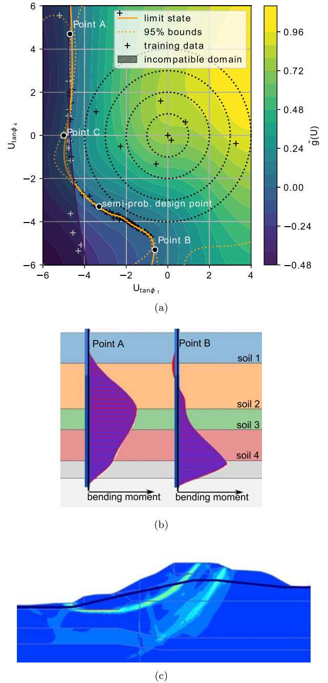
Figure 5. (a) 2D response surface with estimated limit state, limit state 95% confidence bounds, incompatible domain and training datapoints. (b) Bending moment profiles corresponding to Points A and B, with maximum bending moment M_{\max} \approx 279.2 kNm/m' at both A and B. (c) Deviatoric strain contours indicating the failure mechanism for an incompatible realisation at Point C, in the initialisation phase before sheetpile wall installation.
