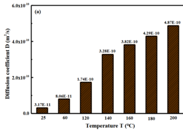
Predicted Diffusion Coefficient D based on MD simulation
