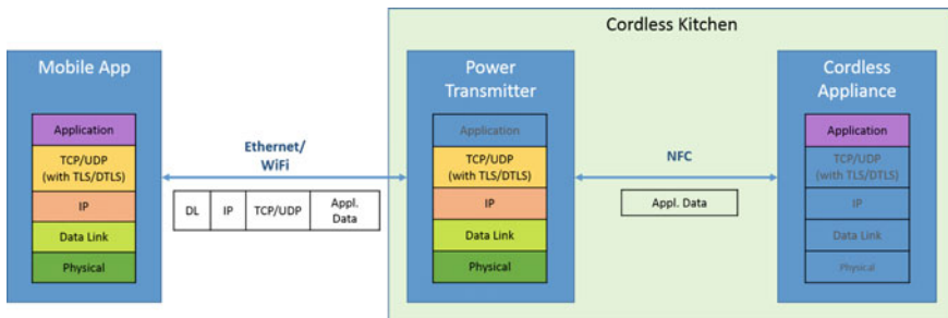
Fig. 3.1 Proxy architecture for Internet connectivity
