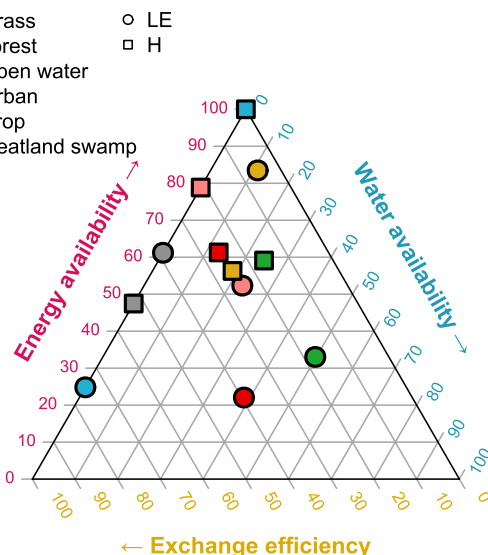
Figure 9. Synthesis of the drivers of latent heat flux (circles) and sensible heat flux (squares) per land cover type at a daily timescale. The data of all sites are merged per land cover type.
