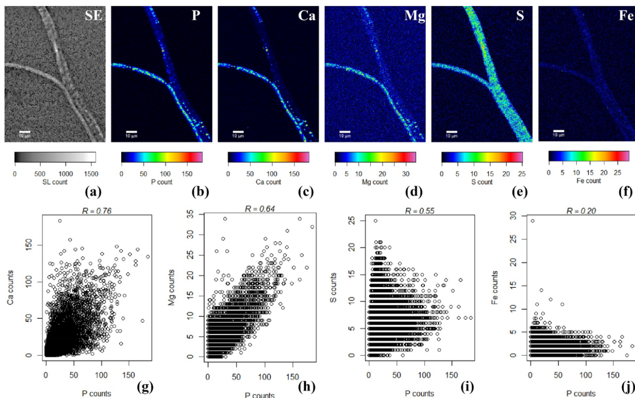
Figure 4. False-colored WDS element maps of (a) secondary electrons, (b) phosphorus, (c) calcium, (d) magnesium, (e) sulfur and (f) iron. Scale bars represent 10 \mu\text{m} . To assess the correlation between the elements, scatterplots of (g) P and Ca, (h) P and Mg, (i) P and S and (j) P and Fe are shown. All scatterplots were produced from a pixel-by-pixel analysis from the WDS X-ray element maps collected with the EPMA. The Pearson's correlation coefficient ( R ) values are depicted on top of the scatterplots. Filaments were extracted from the suboxic zone of sediment incubations from Rattekaai salt marsh.
