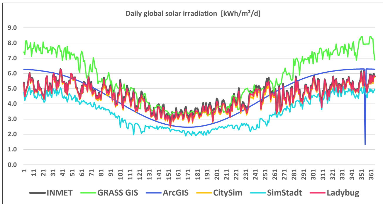
Figure 7. Yearly time series of daily global solar irradiation resulting from the 5 simulation tools and compared to the meteorological station (INMET, in black).
