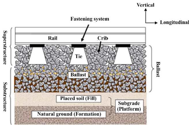
Fig. 1. Components of conventional railway ballasted track [3,5].
