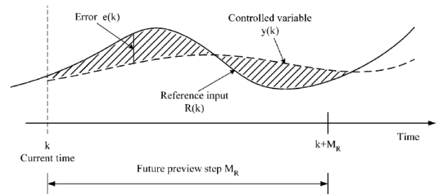
Figure 1. Principle of preview control
