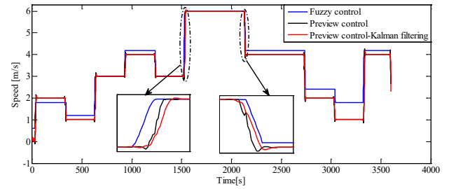
Figure 6. Comparison of speed regulation
