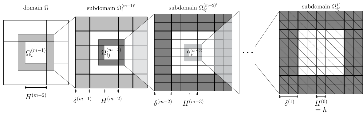
Figure 2: Structured decomposition of a two-dimensional computational domain \Omega into non-overlapping subdomains \Omega_i^{(k)} , a zoom into one overlapping subdomain \Omega_i^{(m-1)'} consisting of subdomains \Omega_{ij}^{(m-2)} (left middle). Furthermore, we show the zoom into one overlapping subdomain \Omega_{ij}^{(1)'} of the first level (right). For all coarser levels ( k > 1 ), the degrees of freedom correspond to vertices \nu_k and edges \varepsilon_k of the non-overlapping decomposition. This figure is based on [18, Figure 1].
