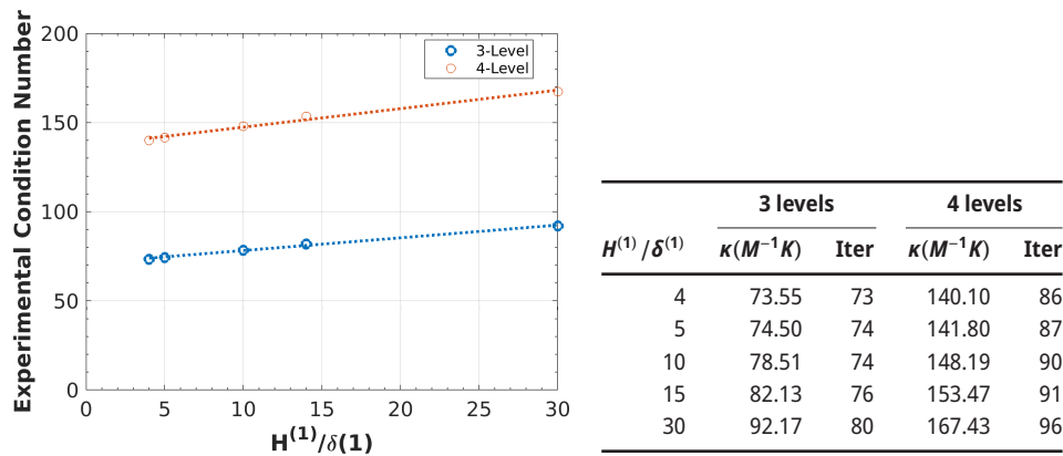
Figure 6: Numerical scalability varying H^{(1)} / \delta^{(1)} for the multilevel GDSW methods with three and four levels. We apply the preconditioner to the two-dimensional Laplace model problem. The number of subdomains on the first level and the number of cores is 4096. We choose H^{(1)} / h = 120 such that the problem size is 58 982 400. The other parameters determining the condition number bound are kept constant such that we have H^{(2)} / H^{(1)} = 4 and H^{(2)} / \delta^{(2)} = 4 . For the fourth level, we chose 16 cores, thus H^{(3)} / H^{(2)} = 4 , and we chose H^{(3)} / \delta^{(3)} = 4 . The dotted line is a least square fit of a linear function to the data.
