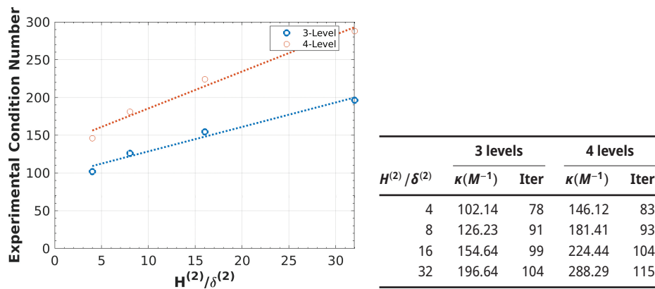
Figure 7: Numerical scalability varying H^{(2)} / \delta^{(2)} for the multilevel GDSW methods with three and four levels. We apply the preconditioner to the two-dimensional Laplace model problem. The number of subdomains on the first level and the number of cores is 16 384. We choose H^{(1)} / h = 80 such that the problem size is 104 857 600. The other parameters determining the condition number bound are kept constant such that we have H^{(2)} / H^{(1)} = 32 and H^{(1)} / \delta^{(1)} = 40 . We choose H^{(3)} / H^{(2)} = 2 . The overlap \delta^{(3)} is chosen such that only the degrees of freedoms on the interface are shared among the processes. The dotted line is a least square fit of a linear function to the data.
