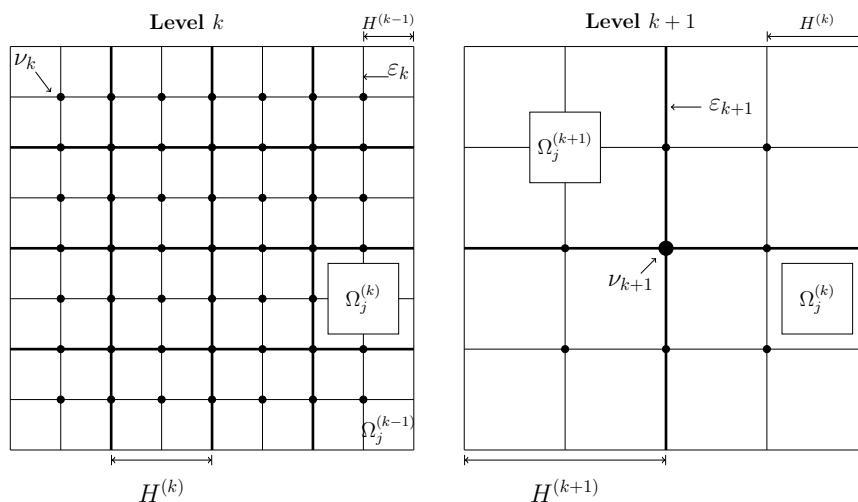
Figure 3: Grid and decomposition into non-overlapping subdomains on the coarser levels k and k+1 . The dots correspond to the vertices and the line segments between the dots to the edges. Note that the dots on level k correspond to the vertices of the decomposition into the subdomains \Omega_j^{(k-1)} . We use the index k since it corresponds to the degrees of freedom on level k .
