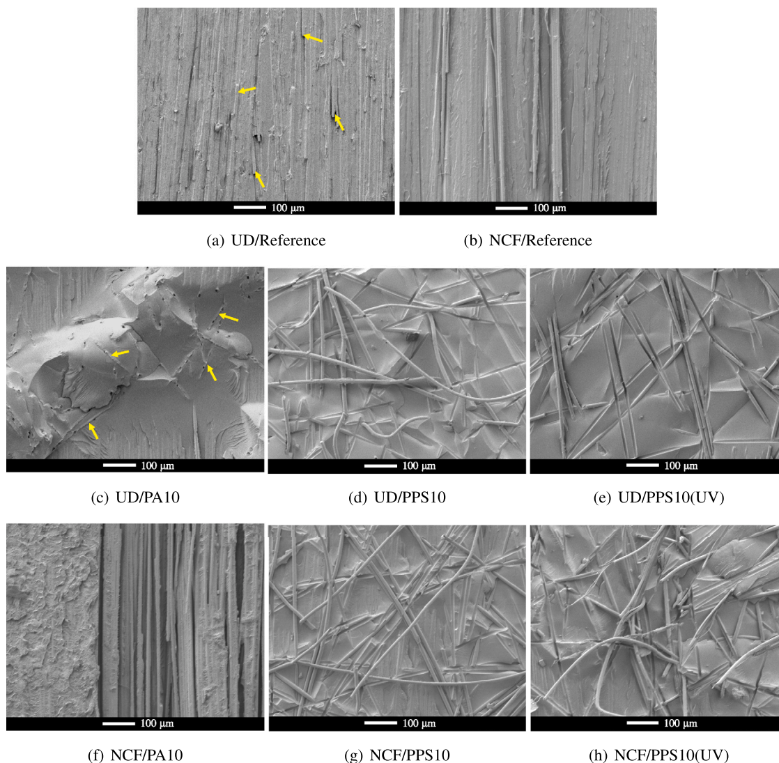
Fig. 7. Representative SEM images of fatigue fracture surface of the DCB specimens. The yellow arrows in (a) and (c) indicate a number of fractured carbon fibres and PA fibres, respectively.
