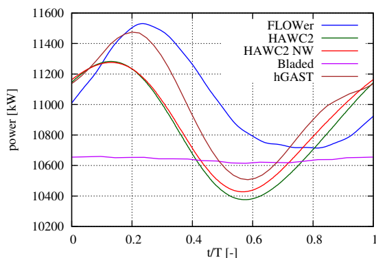
Figure 7. Comparison of rotor power time series over one revolution (11.4m/s - 6p flap).
