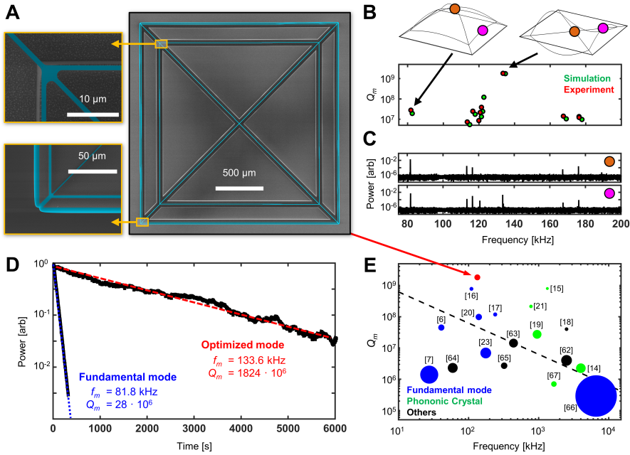
Fig. 3.6 Experimental characterization of the optimal spiderweb nanomechanical resonator. A False-colored scanning electron microscope images of the optimal design. B Q_m from the simulation and experimental results of the out-of-plane vibration modes with the figure of the fundamental and optimized mode shapes. C The thermomechanical noise spectra measured at the center of the resonator (orange marker) and the center of the inner lateral beam (pink marker). The y-axis is the normalized power with respect to the maximum power. D Ringdown measurement of the optimized 3 mm spiderweb resonator excited in its 133.6 kHz mode with an extracted quality factor higher than 1.8 billion, compared with the quality factor measured for the fundamental mode at 81.8 kHz. The y-axis is the normalized power with respect to the power at time=0 for each curve. E Comparison of the presented experiment result with state-of-the-art experiment reports 6,7,14-21,23,63-68 . Marker area corresponds to their aspect ratio t/L . The dashed line corresponds to the mechanical decoherence constraint in Figure 3.1
