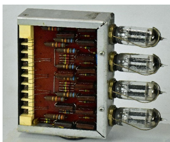
Figure 3. Decade counter built using four double triodes
