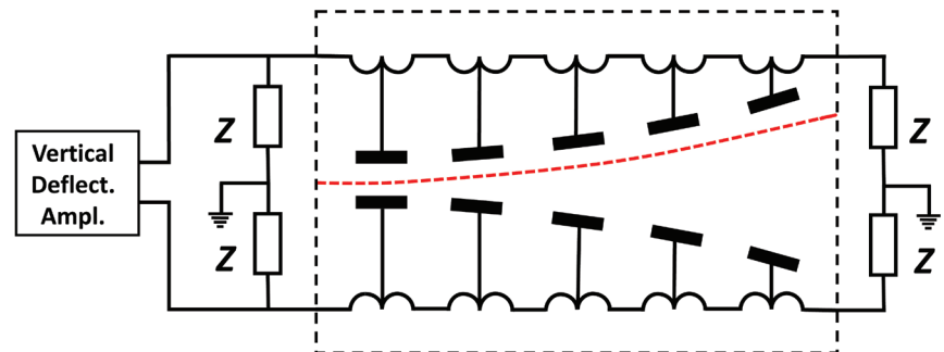
Figure 3. Distributed deflection assembly; the configuration is 'seen' as a transmission line by the vertical amplifier [2]
