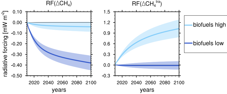
Figure 6.6: Radiative forcing of the impact on methane ( CH_4 ) and of contribution to methane ( CH_4^{tra} ) caused by the scenarios "biofuel low" and "biofuel high". Values indicate the change towards the reference simulation. The time period from 2010 to 2100 is presented. The range of radiative forcings related to the emission uncertainty is displayed as well.
