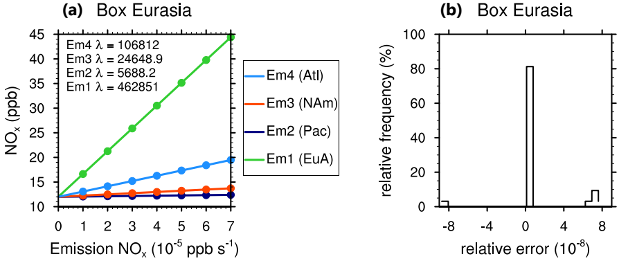
Figure 5.7: (a) \text{NO}_x mixing ratios in box Eurasia depending on an increase of additional \text{NO}_x emissions (Em) in box Eurasia (EuA), Pacific (Pac), North America (NA) and Atlantic (Atl). The dots indicate the data points of the LUT. The regressions coefficients \lambda are also given. (b) Relative frequency distribution of the relative error between the \text{NO}_x mixing ratios determined after eqs. (5.19) and the original values derived from 32 simulations performed with the 4-box-model for all four boxes.
