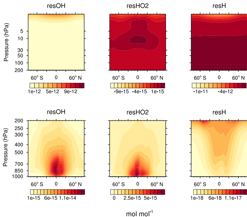
Figure A.3: Zonal mean of rest terms resOH , resHO2 and resH . The first row ranges from 1 to 200 hPa, the second row from 1000 to 200 hPa.
