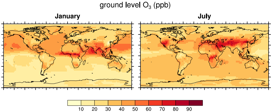
Figure 2.3: Ground level ozone mixing ratios in ppb in January and July for the year 2010. Values are taken from a simulation with the global chemistry climate model EMAC. The model setup and the emission inventory are explained in sect. 3.
