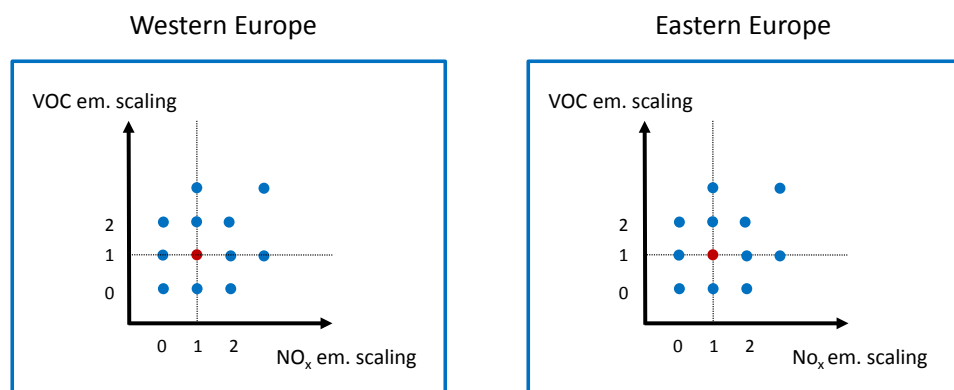
Figure A.5: Resolution of emission variation simulations performed with EMAC for emission regions Western and Eastern Europe. The emission scaling factors for the NO x and VOC road traffic emissions are presented. The reference simulation is indicated with a red dot.
