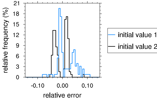
Figure 5.11: Relative frequency distribution of the relative errors of \vec{z} determined after the iteration method. Shown are the distributions for two different initial values.
