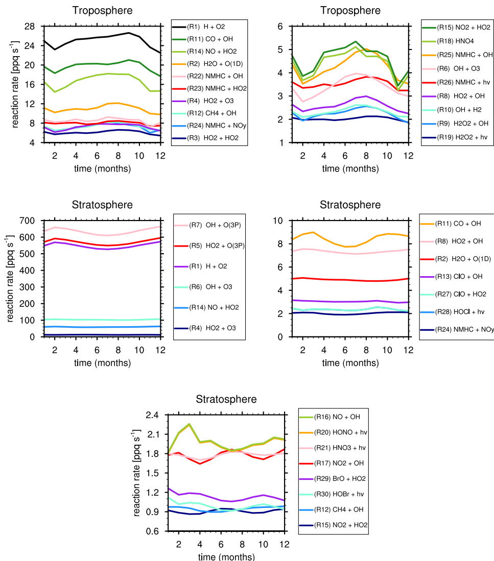
Figure A.2: Reaction rates of HO x reactions with a tropospheric or stratospheric annual mean reaction rate larger than 10^{-15} mol mol -1 s -1 .
