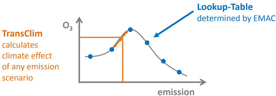
Figure 5.2: TransClim is based on a lookup-table (LUT) determined with the global chemistry climate model EMAC. By interpolating within the LUT TransClim determines the climate effect of any road traffic emission scenario.
