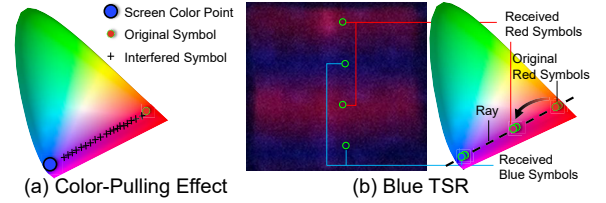
Figure 6: Color-pulling effect caused by the rendering.
