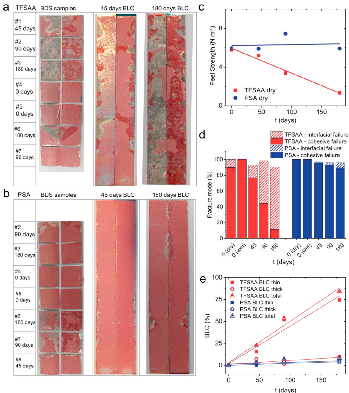
Fig. 5. Representation of opened BDS samples according to their position respect the FRP specimens for TFSA (a) and PSA (b) where the BDS samples, the 45 days BLC specimen and 180 days BLC specimen are shown at the left, middle and right respectively. Individual images show thin adherend present on the thin (left) and thick (right) adherends of each sample. (c) Peel strength of the panels TFSA and PSA after exposure times of 0, 45, 90 and 180 days. (d) Fracture modes of the panels, determined by visual analysis of the surfaces highlighting the distribution of the different failure modes. (e) BLC results for panels TFSA and PSA as function of exposure time show more corrosion in the thin adherend panel of the TFSA sample.
