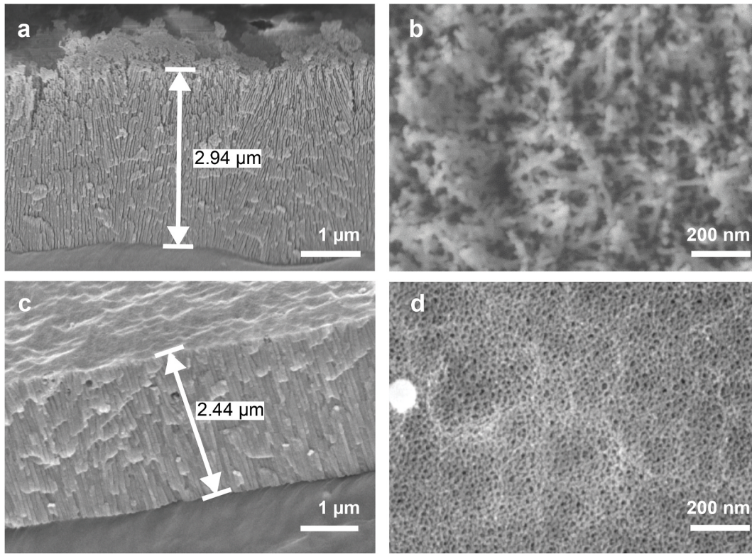
Fig. 2. SEM images of the surface morphology of the oxides produced with PSA (a for side view and b for top view) and TFSA (c for side view and d for top view).
