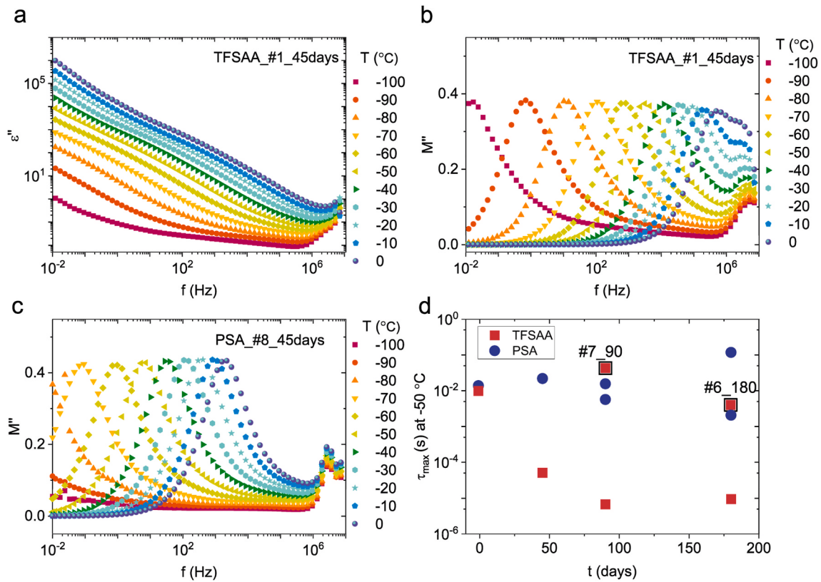
Fig. 4. (a) Dielectric loss permittivity of sample TFSA #1_45days shows dominant electrode polarization. By using the modulus formalism, large values of permittivity and conductivity can be suppressed as shown in (b) TFSA #1_45 days and (c) PSA #8_45days. Apparent conductivity relaxation times ( \tau_{max} at -50\text{ }^{\circ}\text{C} ) for panels TFSA and PSA as function of exposure time (d). Samples TFSA #7_90 and TFSA #6_180 highlighted with black squares show comparable results to PSA samples for the same exposure time in good agreement with comparable states of the fractured surfaces shown in Fig. 5.
