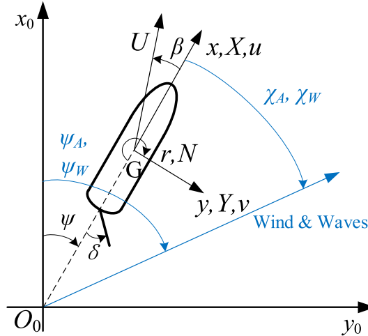
Fig. 4. Coordinate system of MMG manoeuvring model, and wind &amp; waves.
