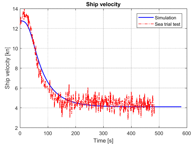
(b) Ship velocity - time
