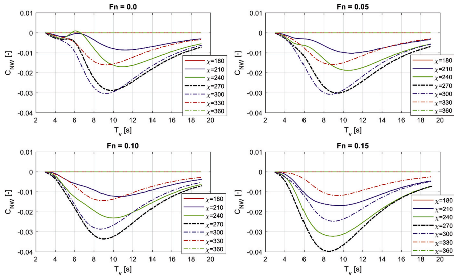
Fig. A.1. Averaged steady forces and moments coefficients of S-Cb84 in irregular waves calculated using SKFM (Yasukawa et al., 2019)
