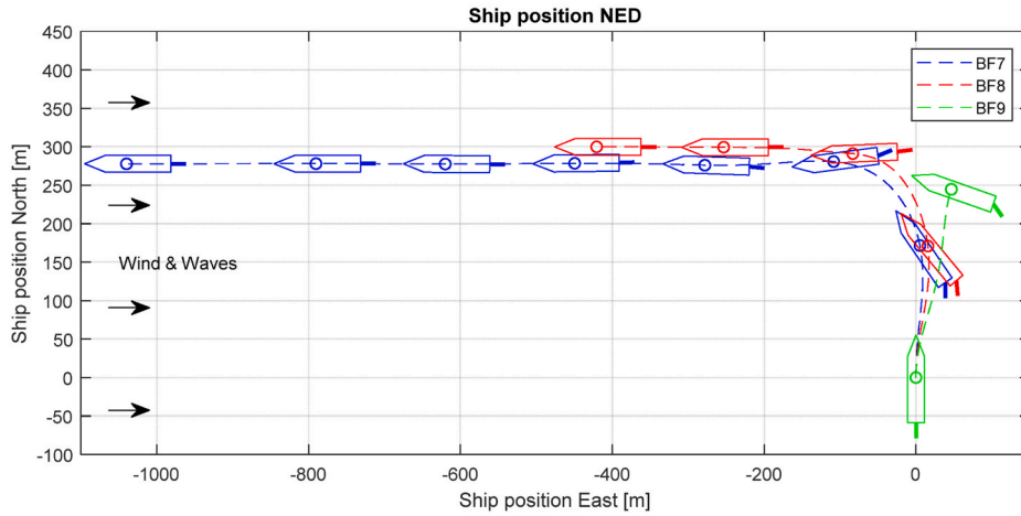
(b) Ship position trajectory during turning to head sea
