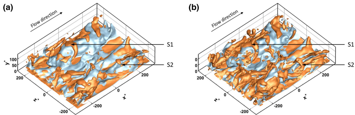
Fig. 6 Instantaneous flow organization in the measurement volume visualized by isosurfaces of vorticity magnitude ( |\omega^+| = 0.3 , orange) and streamwise velocity ( u^+ = 14 , blue). Tomographic PIV (a) and VIC+ (b)
