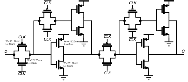
Fig. 4. D-flip-flop with specific sizing implementing measures (A), (B), (C), (D), and (E), as described in the text.
