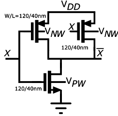
Fig. 3. Schematic of the 1X strength inverter cell.
