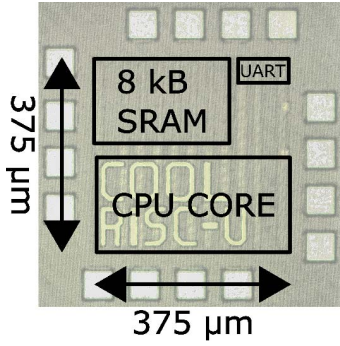
Fig. 6. Micrograph of the RISC-V chip fabricated in a standard 40-nm CMOS process.
