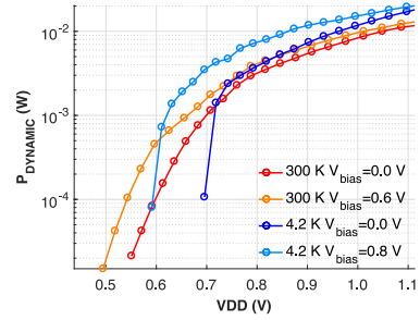
Fig. 11. Dynamic power in the RISC-V.
