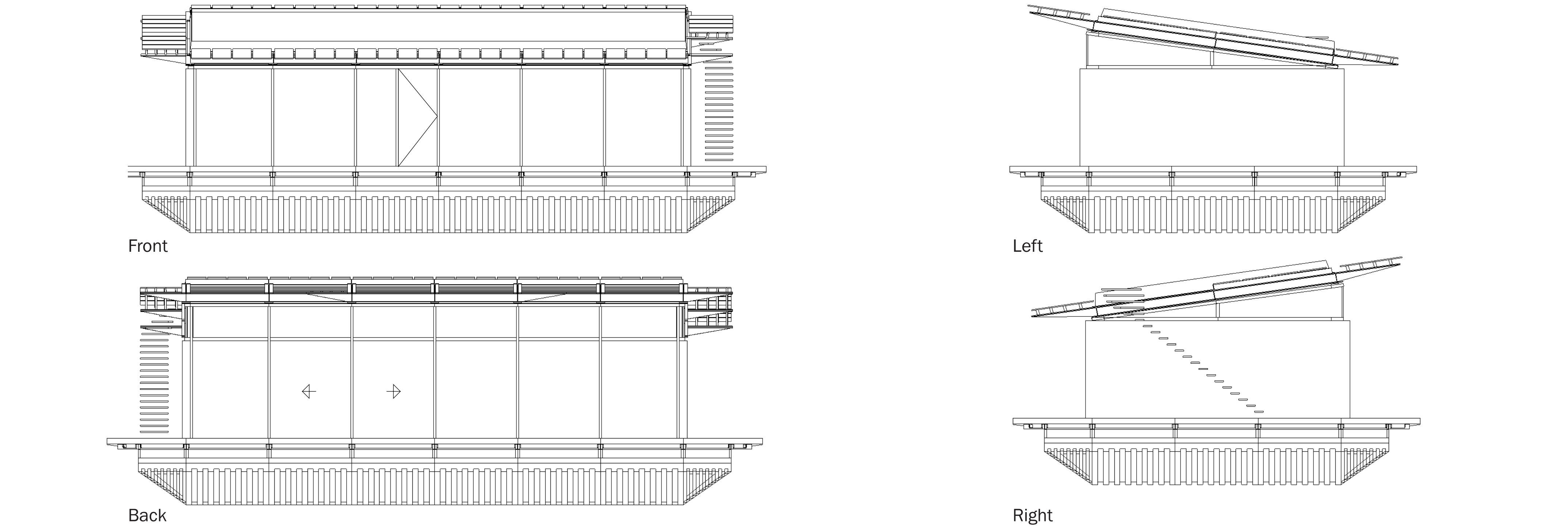
Elevations
