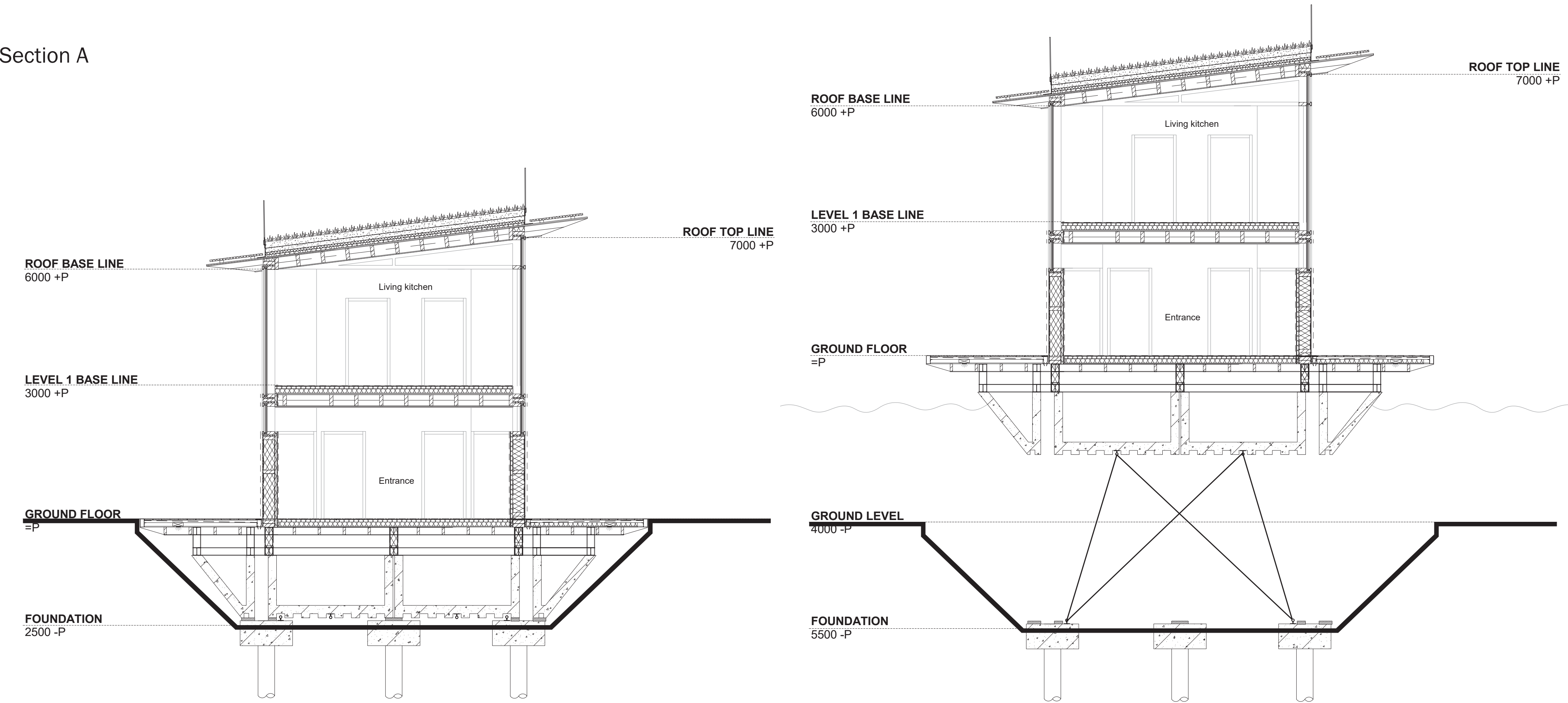
Elevations
