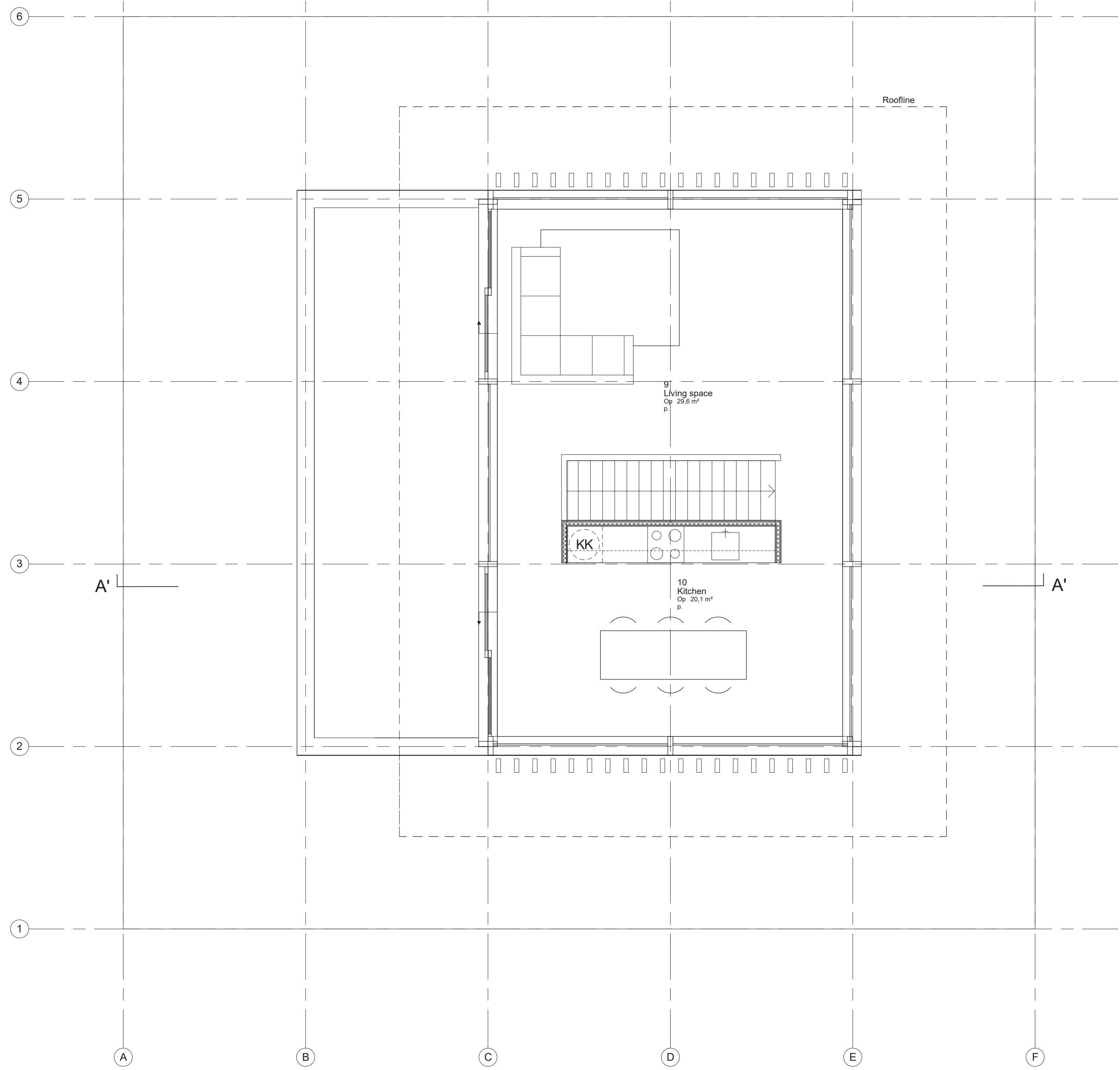
Floorplan first floor 1:50
