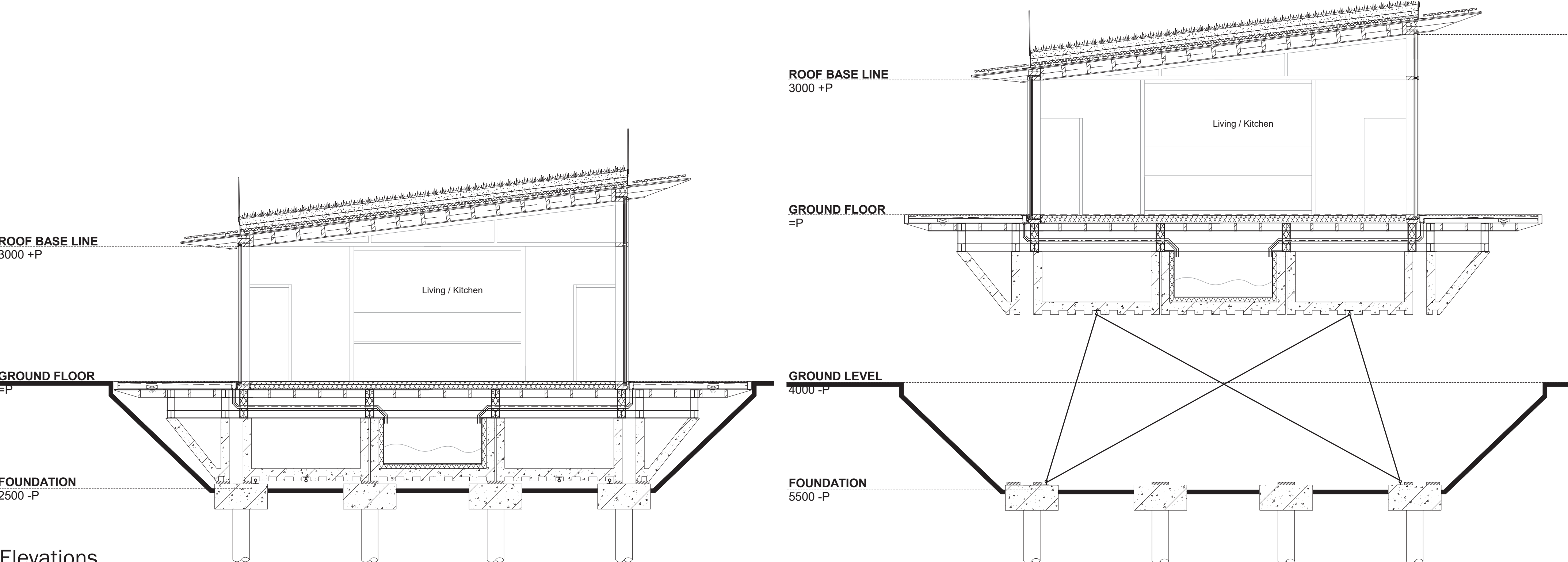
Elevations
