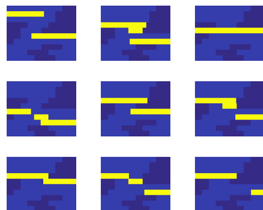
Figure 25 Nine arbitrary permeability models taken from the ensemble of 40 model realizations.
