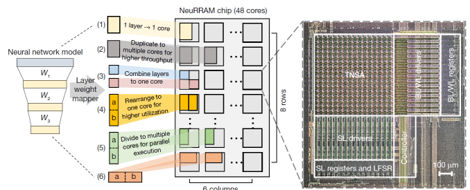
Figure 4. RRAM-based CIM chip and its NeuRRAM embedding [6].
