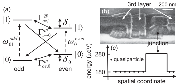
FIG. 1. (a) Low energy-level structure of a transmon qubit. The parity state with larger separation between |0\rangle and |1\rangle qubit states is assigned to odd without loss of generality. \delta_0 and \delta_1 : Energy difference between odd-even parities for the ground and first excited state, respectively, \delta_1 \gg \delta_0 . \omega_{01}^{\text{odd}} - \omega_{01}^{\text{even}} = \omega_{oe} \approx \delta_1 is the charge dispersion. \Gamma_{oe,i}^{qp} is the switching rate between qubit states of different parities. \Gamma_{1\rightarrow 0}^{qp} \approx \Gamma_{1e\rightarrow 0o}^{qp} = \Gamma_{1\rightarrow 0}^{qp} is the qubit relaxation rate because \omega_{01}^{\text{odd}} \approx \omega_{01}^{\text{even}} = \omega_{01} \gg \delta_1 . (b) SEM image of a typical device fabricated by three-angle evaporation to engineer the band gap profile. (c) Expected band gap profile near the tunnel junction.
