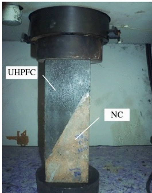
Fig. 12. Slant shear test set-up for UHPC-NC specimen [89].
