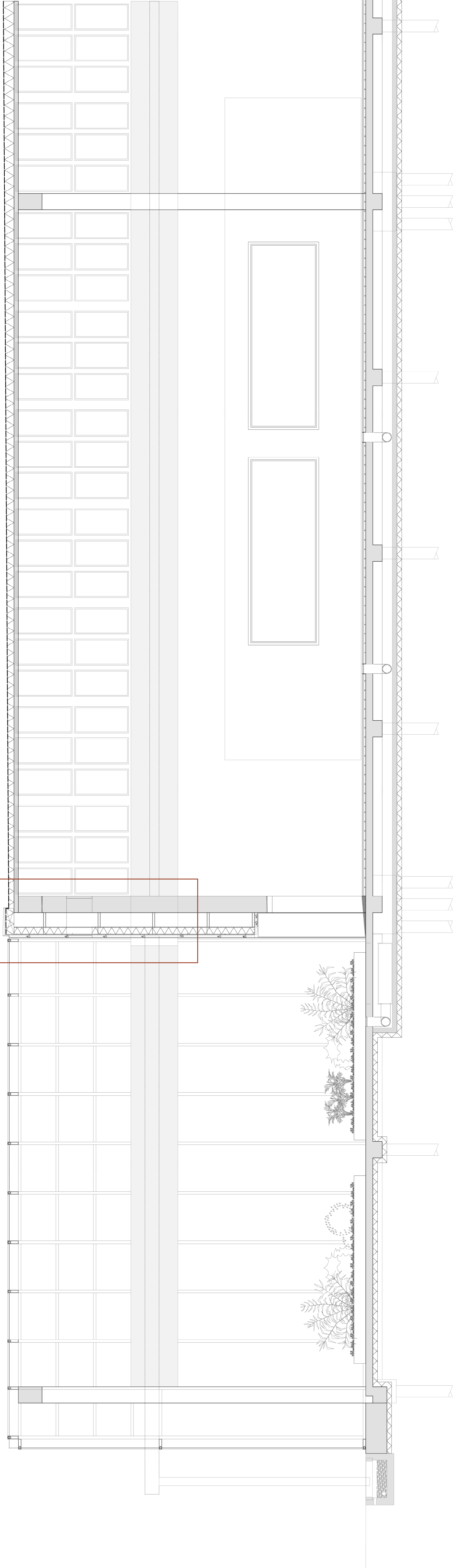
Section B
