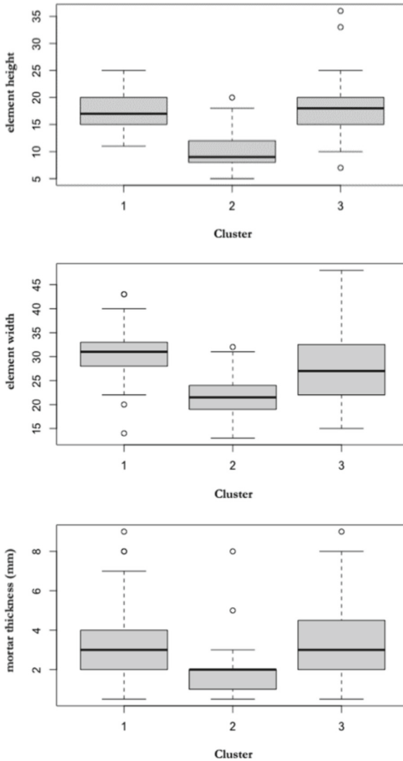
Fig. 10. Boxplots of geometric dimensions within the 3 clusters (a) element height (b) element width (c) mortar thickness © 2024, by authors.
