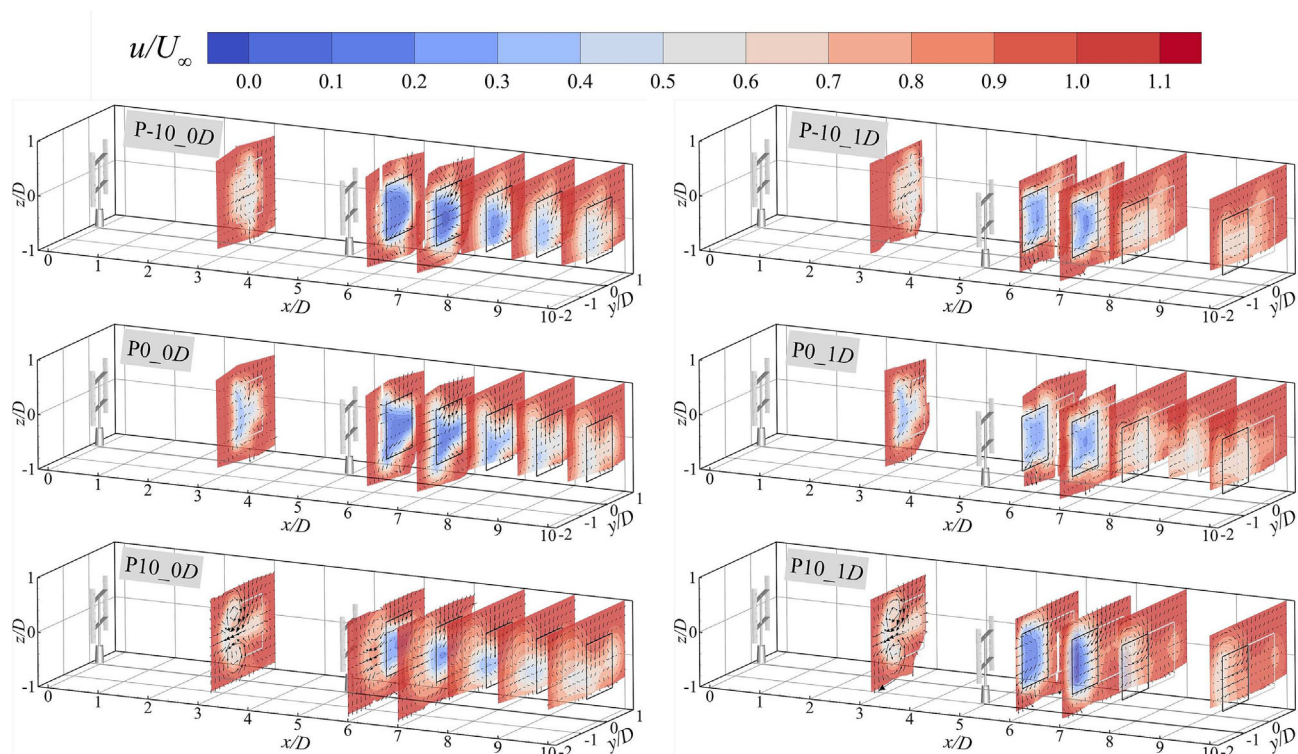
FIGURE 6 Overview of the placement of the turbine and measured streamwise velocity contours. Grey squares denote the frontal area of the upwind turbine (VAWT1) while black squares for the downwind turbine (VAWT2).
