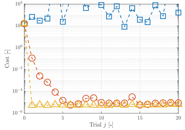
Figure 3. Error norm per trial j for the commutative SK-based approach (—□—), the experimentally intensive MIMO RBF approach (—○—), and the experimentally efficient MIMO RBF approach (—△—) for the case of no model mismatch. Clearly, the later converges almost instantly and monotonically.
