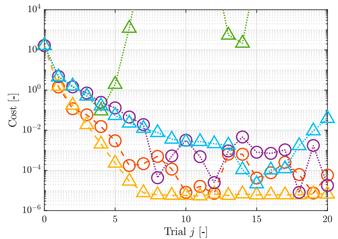
Figure 7. Error norm per trial j . The experimentally intensive approach for light ( \ominus ) and severe ( \ominus ) model mismatch shows that the latter converges more slowly, but still attains a low cost for certain trials without increasing regularisation. The experimentally efficient approach for severe model mismatch ( \triangle ) and for increased regularisation ( \triangle ) highlight the importance of regularisation, and the latter converges towards a slightly higher error norm, albeit at a slower rate, compared to the light model mismatch case ( \triangle ).
