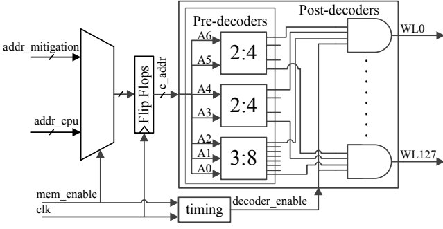
Fig. 4: Address decoder mitigation scheme.
