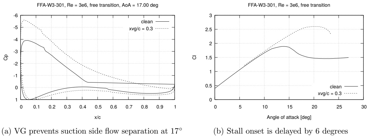
Figure 2: A VG placed at x/c = 0.3 on an FFA-W3-301 airfoil delays flow separation and stall.
