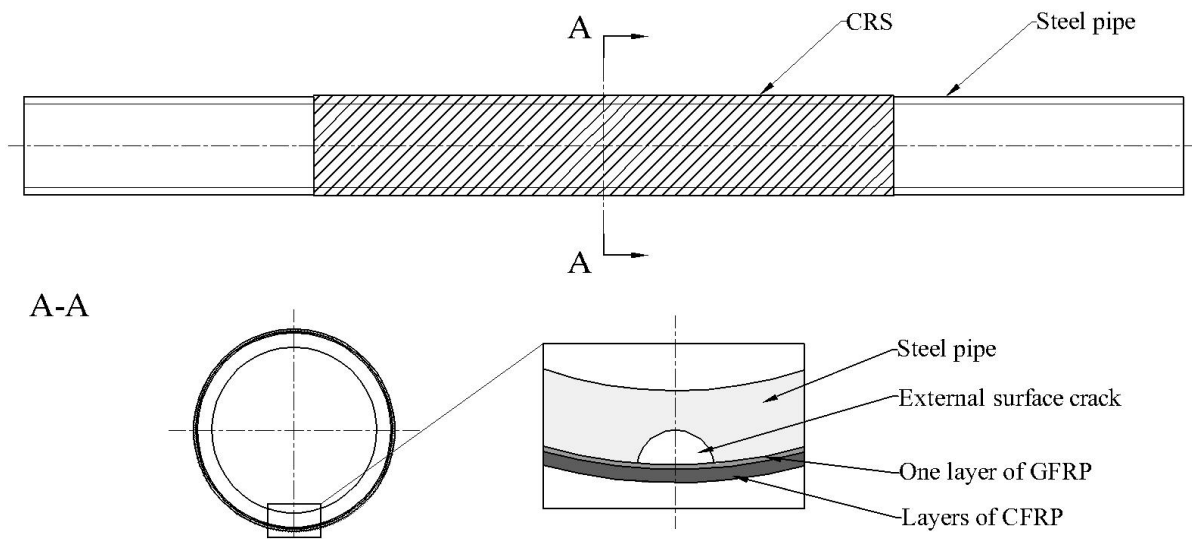
Figure 6.2. The configuration of composite reinforced steep pipe specimens
