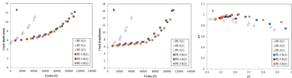
Figure 6.12. The experimental results of PE-3 and PE-3-R of using the default reinforcement scheme: a) crack growth along depth direction; b) crack growth along length direction; c) aspect ratio variation: a/c versus a/t curves
