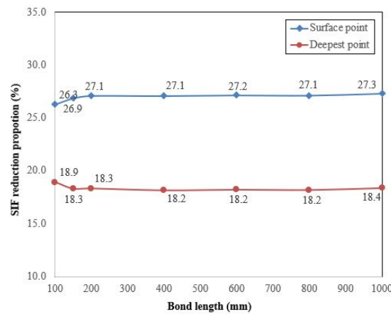
Figure 6.34. The SIF reduction results of the deepest point and the surface point with different bond length
