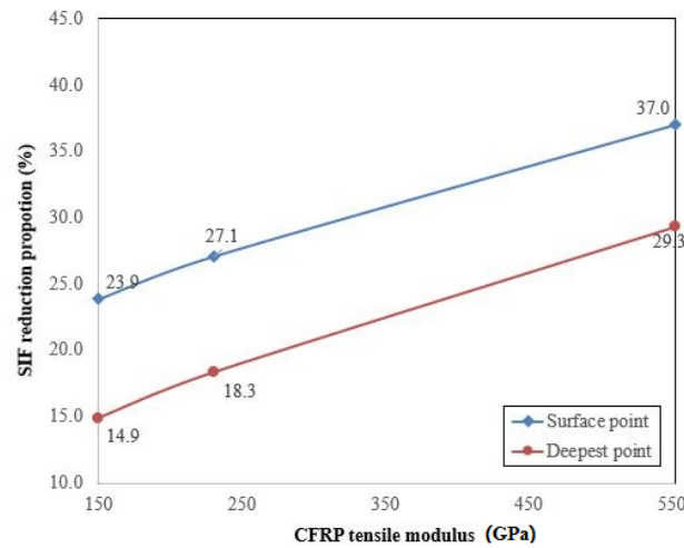
Figure 6.36. The SIF response of the FE models with different CFRP tensile modulus: a) the normalised SIF result along the crack front; b) the SIF reduction proportion of the deepest point and the surface point
