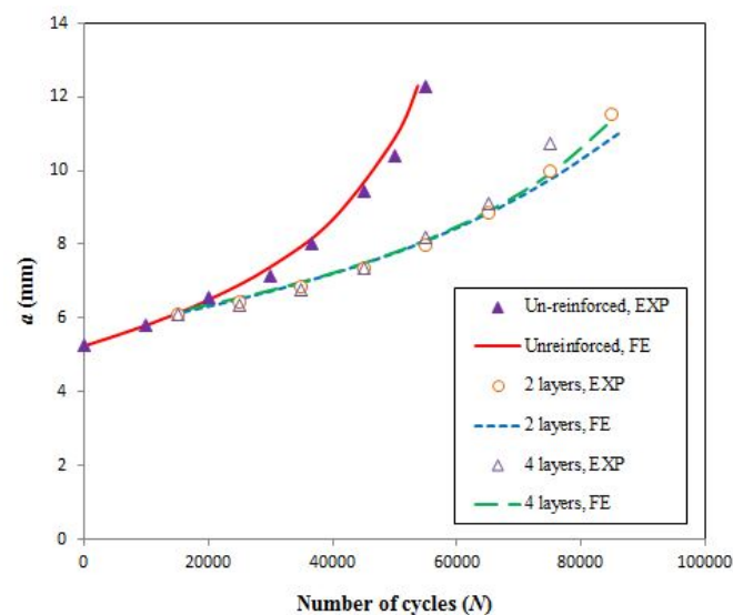
Figure 4.41. The FE and experimental results of the cracked plate by using two layers and four layer of CFRP respectively
