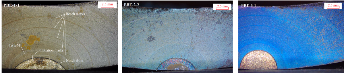
Figure 3.16. Beach marks on the cross-section of three pipe bending specimens
