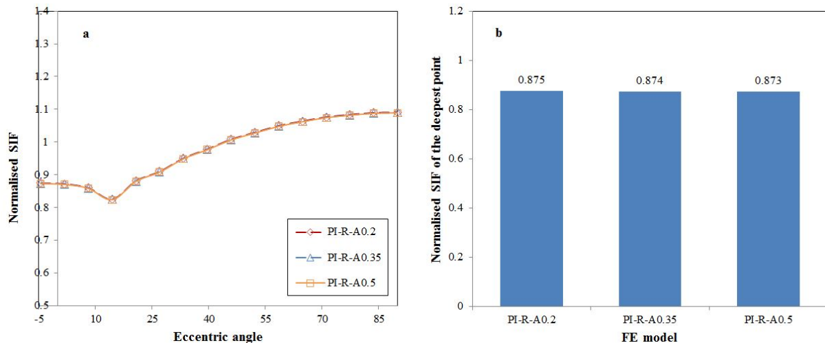
Figure 5.17. The normalised SIF result of FE models with different adhesive thickness: a) normalised SIF along the crack front; b) normalised SIF of the deepest point
