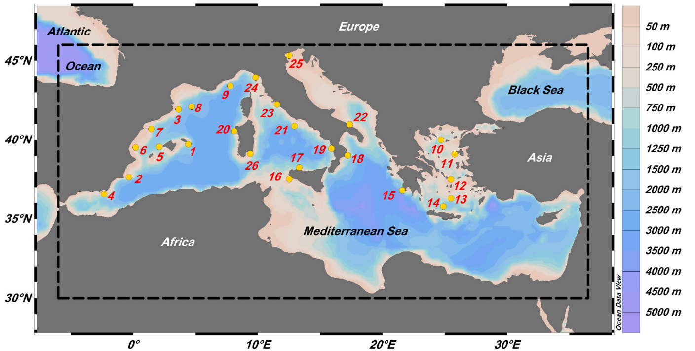
Fig. 2. Study area showing the model domain (the dashed rectangle), bathymetry and the locations of the wave buoys are shown in yellow circles and numbered in red.
