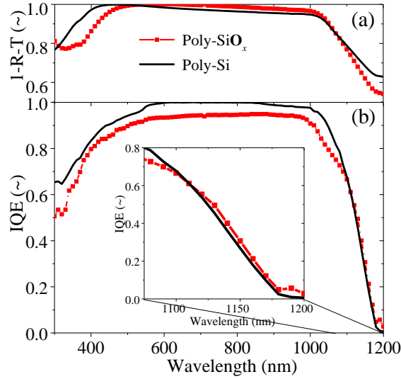
FIG. 5 (a) Reflectance ( R ) and transmittance ( T ) of both cells are plotted as 1-R-T. (b) The internal quantum efficiency (IQE) of the best IBC solar cell with either poly-SiO x or poly-Si as carrier-selective passivating contacts for both polarities. The inset in (b) zooms-in the long wavelength region.
