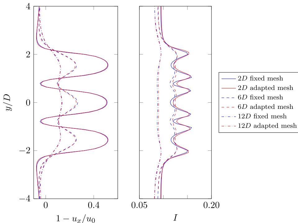
Fig. 15. Lateral velocity deficit and turbulence intensity plots at x = 2D , x = 6D and x = 12D with z = 0 showing the results from both the fixed mesh and the adaptive mesh simulations using the Fluidity k - \omega SST model with C_T = 0.92 .
