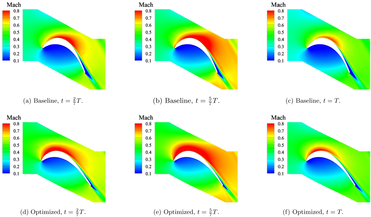
Fig. 15. Mach number contours calculated at three different time instances with the HB method, based on the OptC2 test case, for both the baseline (a), (b), (c) and the optimized (d), (e), (f) blade profile.
