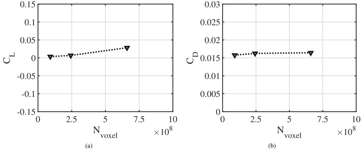
Fig. 12 Trends of the time-averaged (a) lift coefficient C_L and (b) drag coefficient C_D , integrated along the airfoil surface, at the three different resolution configurations for the NACA-0012 case.
