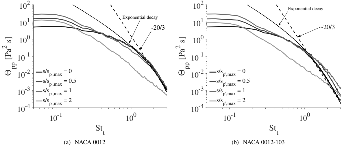
Fig. 5 Surface-pressure spectra at the airfoil leading edge. The distances along the airfoil surface have been set as multiples of the curvilinear abscissa s_{p',max}/c where the root-mean-square of the surface-pressure fluctuation is maximum.
