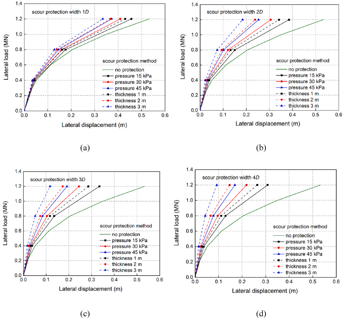
Fig. 5. Lateral load-lateral displacement relationships under four scour protection widths from FEA: (a) 1D, (b) 2D, (c) 3D, and (d) 4D.
