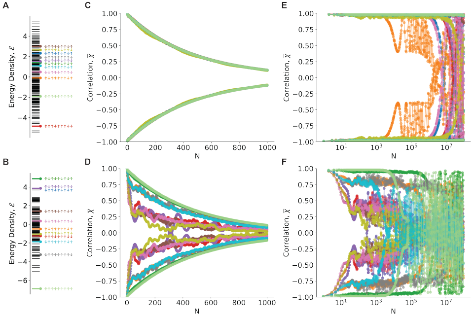
Figure 7.10: Initial state dependence (A and B) Calculated energy densities \mathcal{E} for all possible states of the form \bigotimes_j^L |m_j\rangle , m_j \in \{\uparrow, \downarrow\} (black lines), for the disordered experimental Hamiltonian (Table 7.2, A) and a theoretical disorder-free Hamiltonian (Table 7.6, B). The initial states measured in Fig. 7.4D are indicated by the corresponding colors. (C and D) Simulated values of the correlation function \bar{\chi} for the 11 initial states used in the experiments, up to N = 1000 Floquet periods, with (C) and without (D) disorder. The simulated results are multiplied by the decay function f(N) = Ae^{-N/N_{1/e}} , with N_{1/e} = 472(17) extracted from a fit to the experimental data (Fig. 7.4D). Clear behavioural differences can be observed within the experimentally accessed timescales. (E and F) Simulated values of the correlation function \bar{\chi} up to N = 10^8 Floquet periods, with (E) and without (F) disorder.
