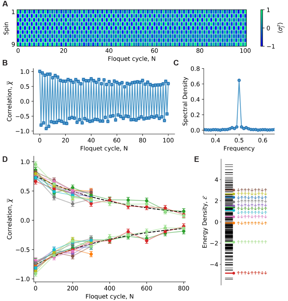
Figure 7.4: Observation of the DTC response for generic initial states. (A) Individual spin expectation values \langle \sigma_z^j \rangle as a function of N after initialising the spins in the Néel state |\uparrow\downarrow\uparrow\downarrow\uparrow\downarrow\uparrow\rangle and applying U_F for \theta = 0.95\pi and \tau = 5 ms. (B) Averaged two-point correlation function \bar{\chi} , corresponding to the data in (A). The DTC response persists to similar high N as for the polarised state (Fig. 7.3B). (C) Fourier transform of the data in (B), showing the period-doubled response. (D) Average correlation for even (upper curve) and odd (lower curve) N for 9 randomly chosen initial states, plus the polarised state and the Néel state (indicated in (E)) with \theta = 0.95\pi and \tau = 5 ms. Each data point is the average over even/odd integers in the range N to N + 10 . Three of the states are measured up to N = 800 , the others to N = 300 . The dashed black line is a fit of |\bar{\chi}| , averaged over the three states measured to N = 800 , using a phenomenological function f(N) = Ae^{-N/N_{1/e}} , giving A = 0.76(1) and N_{1/e} = 472(17) . (E) Calculated energy density \mathcal{E} for all possible states of the form \bigotimes_j^L |m_j\rangle , m_j \in \{\uparrow, \downarrow\} (black lines). The initial states measured in (D) are indicated by the corresponding colors.
