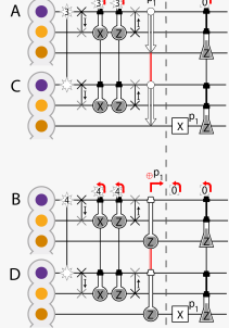
Figure 4.12: Circuit diagrams of the three GHZ creation protocols used in the simulations. Bell states are generated in the form of Eq. 4.8, followed by an X-gate on their second qubit to turn them into noisy versions of the (|00\rangle + |11\rangle)/\sqrt{2} state. ‘Plain’ uses three Bell pairs to create a 4-qubit GHZ state. ‘Modicum’ uses a fourth Bell pair to increase the GHZ fidelity with a distillation step. ‘Expedient’ 2 uses 22 Bell pairs and has many (intermediate) distillation steps. Details of those steps are given in the text. The schematics above the circuits show four network nodes (A,B,C,D) comprising an electron spin (purple) and up to three nuclear spins (orange tones).
