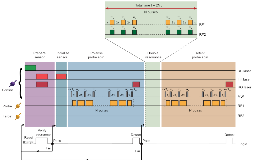
Figure 6.5: Experimental sequence. The pulse sequence consists of five parts: sensor preparation, sensor initialisation, polarisation of the probe spin, double resonance, and detection of the probe spin. Sensor preparation: The NV centre is prepared by excitation with two 637 nm lasers for 150 \mu\text{s} and counting the detected photons (RO laser resonant with the E_x transition and Init laser with the E' transition) 25,35 . If the number of photons exceeds a certain threshold, the NV is in the negative charge state and resonant with both lasers, and we proceed to the next step. If not, we apply a 515 nm laser (charge reset (RS) laser, 1 ms) and repeat the process 25,35 . Sensor initialisation: The NV electron spin is initialised into the m_s = 0 state through spin pumping (Init laser, 100 \mu\text{s} ) 35 . Polarising probe spin: First, the NV sensor is brought into a superposition state using a \pi/2 pulse. Then, a dynamical decoupling sequence of N' equally spaced \pi -pulses on the electron spin of the form (\tau_r - \pi - \tau_r)^{N'} is applied. This sequence correlates the state of the nuclear spin(s) with the phase of the electron spin. We use two different sequences (see Sec. 6.7.3). For sequence B, the MW \pi -pulses are interleaved with radio-frequency pulses (RF1) that resonantly drive the probe spin(s) (dashed box), see Bradley et al. for details 29 . A second \pi/2 pulse maps the electron phase to population and the electron spin is read out (RO laser). Double resonance: N echo pulses are applied simultaneously on the probe spin(s) (RF1) and the target spin(s) (RF2), so that the coupling between these spins is isolated. To mitigate pulse errors we alternate the phases of the pulses following the XY8 scheme 43 . Detecting probe spin: The detection sequence is the same as the polarisation sequence except for the final RO laser pulse which is applied for 10 \mu\text{s} and with higher power.
