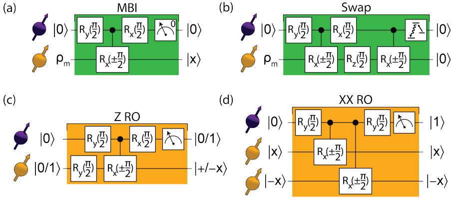
Figure 2.10: Quantum circuits for ^{13}\text{C} initialisation and read-out: For all circuits, the output states correspond to the result of the sequence applied to the corresponding input states, assuming perfect operations. (a) Measurement-based initialisation. This sequence of gates maps the x-basis spin projection of the nuclear-spin to the z-basis of the electron, after which a measurement heralds the |x\rangle nuclear state conditioned on the outcome '0'. (b) Swap initialisation. Compared with (a), an additional single-qubit gate and two-qubit gate realise a partial-swap operation of the electron and nuclear spin states, deterministically preparing the nuclear spin in the |0\rangle state without the need for conditioning on measurement. Finally, the electron spin is reset. (c) Z-basis nuclear-spin read-out. Following the same protocol as in (a), but with an additional single-qubit operation to map the nuclear-spin z-basis to the x-basis for read-out, and utilising full (unconditional) measurement of the electron spin to reveal the nuclear state. (d) Multi-qubit read-out of the XX operator. Concatenating two-qubit gates between the electron and two separate nuclear spins within the sequence reveals information about the joint state of the two nuclear spins. In this case, the XX-parity is odd, and so the electron spin outcome is |1\rangle .
