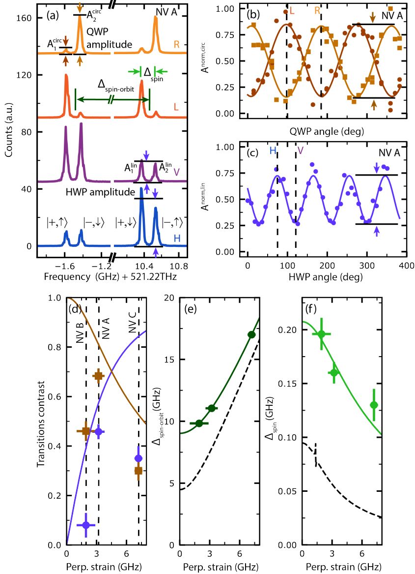
Figure 3.7: Extraction of finestructure constants. (a) PL spectra for four different excitation light polarisations (R, L, V, H) for NV A. (b) NV A: Example traces for extracted and normalised PL amplitudes A_1^{\text{circ, norm}} (circles) and A_2^{\text{circ, norm}} (squares) for varying angles of the quarter-wave plate (QWP). (c) Same as (b) but for A_1^{\text{lin, norm}} and A_2^{\text{lin, norm}} when varying the angle of the half-wave plate (HWP). The dashed lines in (b,c) indicate the angles for which the PL scans in (a) are taken. Solid lines show fits with a sine function. (d) Transition contrast for circular ('orbit contrast', squares) and linear ('spin-orbit contrast', circles) polarisation extracted from the normalised amplitudes, as indicated by the vertical arrows in (b,c), determined for three NV centres (dashed lines). (e,f) \Delta_{\text{spin-orbit}} and \Delta_{\text{spin}} for the same NV centres as in (d). The data of (d-f) is simultaneously fitted against the Hamiltonians. The data is shown together with the best fit (solid lines) as a function of perpendicular strain \epsilon_{\perp} . Dashed lines in (e,f) show the expected transition energy splittings for the fine structure constants of Barson et al. , see Ref. 16 .
