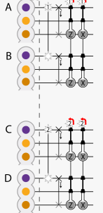
Figure 4.12: Circuit diagrams of the three GHZ creation protocols used in the simulations. Bell states are generated in the form of Eq. 4.8, followed by an X-gate on their second qubit to turn them into noisy versions of the (|00\rangle + |11\rangle)/\sqrt{2} state. ‘Plain’ uses three Bell pairs to create a 4-qubit GHZ state. ‘Modicum’ uses a fourth Bell pair to increase the GHZ fidelity with a distillation step. ‘Expedient’ 2 uses 22 Bell pairs and has many (intermediate) distillation steps. Details of those steps are given in the text. The schematics above the circuits show four network nodes (A,B,C,D) comprising an electron spin (purple) and up to three nuclear spins (orange tones).
