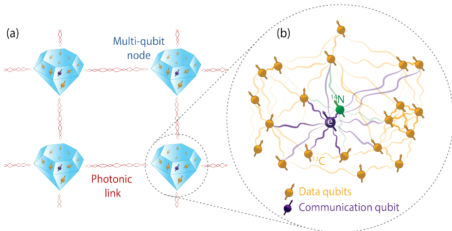
Figure 1.1: Architecture for distributed quantum information processing using spins in diamond. (a) Each diamond node hosts at least one optically-active defect (purple spin, 'Communication qubit'), such as an NV centre as used in this thesis. Coherently emitted photons are interfered to create entanglement between remote electron spins ('Photonic link'). The presence of additional spin qubits within each node, such as ^{13}\text{C} nuclear spins (yellow spins, 'Data qubits'), provides a resource for the manipulation and storage of complex quantum states. The four nodes shown here serve as a unit-cell for a large scale system operating a distributed surface code for quantum error correction 34,69,70 . (b) Schematic of a quantum network node based upon an NV centre within an interacting nuclear spin bath. The central electron spin (purple) exhibits magnetic couplings (purple lines) to the intrinsic ^{14}\text{N} spin of the NV centre (green), and to proximal ^{13}\text{C} spins in the diamond lattice (yellow). Prior to the work of this thesis, a few of the most strongly-coupled ^{13}\text{C} spins (dark purple lines) had been controlled as prototype qubits. In this thesis, we will explore the larger spin environment by first developing techniques to address ^{13}\text{C} spins with weaker electron-nuclear couplings (light purple lines). We will then investigate the couplings between nuclear spins themselves (yellow and green lines) and utilise these for further qubit control. These techniques provide access to spin registers comprising tens of qubits as a resource for quantum technologies. Figure (b) adapted from Aboeish 79 .
