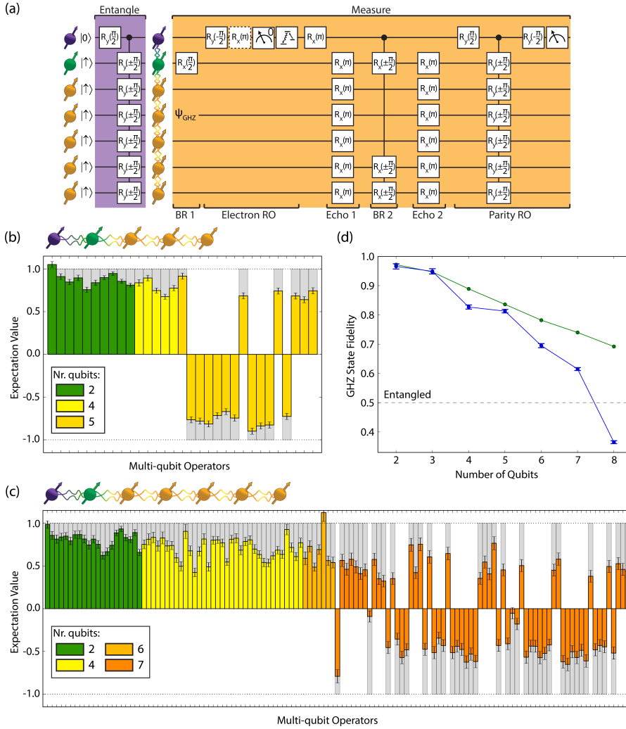
Figure 5.7: (a) Experimental sequence to prepare a 7-qubit GHZ state |\text{GHZ}_7\rangle (purple) and determine the expectation value of the 7-qubit operator XYYYYYZZ (orange). The measurement sequence is broken down into basis rotations (BR 1,2), an electron readout (RO), nuclear spin echoes (Echo 1,2), and a multi-qubit readout of the nuclear spins. All operations are applied sequentially (in the same way as shown in Fig. 5.5), but some are shown in parallel for clarity. (b-c) Bar plots showing the measured expectation values (non-zero terms of the ideal state only) after preparing the 5-spin (b) and 7-spin (c) GHZ states. The colors indicate the number of qubits involved, i.e. the number of (non-identity) operators in the expectation value (inset). Gray bars show the ideal expectation values. See Sec. 5.8.5 for the operator corresponding to each bar. The fidelity with the target state is 0.804(6) (b) and 0.589(5) (c), confirming genuine multipartite entanglement in both cases. (d) Plot of GHZ state fidelity against the number of constituent qubits. A value above 0.5 confirms genuine N -qubit entanglement. The blue points are the measured data, while the green points are theoretical predictions assuming a simple depolarizing noise model whose parameters are extracted from single- and two-qubit experiments. Numerical values are given in Sec. 5.8.5.
