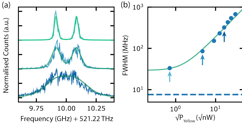
Figure 3.6: Power broadening of \text{NV}^0 optical transitions. (a) Example PL spectra for the lower spin-orbit branch, measured at powers of 0.5 nW, 22 nW, and 160 nW (light to dark blue) with H polarisation. Each spectrum consists of 20 individual scans which have been shifted on top of one another and summed. A pair of Voigt profiles is fitted. The spectra have been normalised and offset for clarity. (b) FWHM of the fitted Voigt profiles, as a function of \sqrt{P_{\text{yellow}}} . The solid line is a fit to the data (see text), from which we extract a = 18.6(1) \text{ MHz}/\sqrt{\text{nW}} and b = 25.1(3) \text{ MHz} . The transform limit, 7.6 MHz, arising from the excited state lifetime, \tau_{\text{exc}} = 21 \text{ ns} , is shown as a dashed line.
