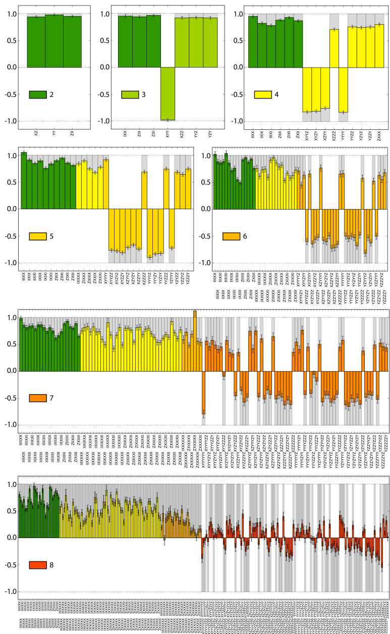
Figure 5.16: Bar plots showing the non-zero expectation values for 2-8 qubit GHZ states, used to calculate the GHZ state fidelity plotted in Fig. 5.7(d). The colors indicate the number of qubits involved, i.e. the number of (non-identity) operators in the expectation value (inset). Gray bars show the ideal expectation values.
