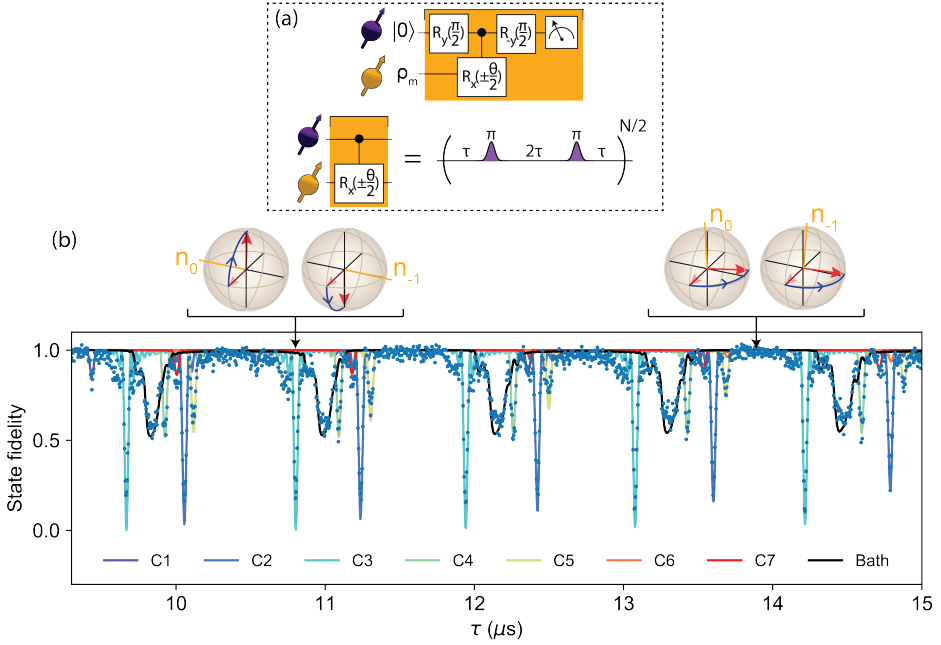
Figure 2.9: Dynamical decoupling (DD) spectroscopy: (a) Quantum circuit for DD spectroscopy. At particular \tau values, a dynamical decoupling sequence of N \pi pulses realises entangling interactions with individual nuclear spins (controlled- R_x(\pm\theta/2) gates, Eq. 2.10), resulting in a loss of coherence (see text). (b) Measured DD spectrum for N = 32 at a magnetic field of 403 G. Solid lines are fitted signals for seven individual ^{13}\text{C} spins and a bath of 200 generated spins with sampled hyperfine couplings < 10 kHz 64 . Bloch spheres presented above the data show the nuclear spin rotation axes \mathbf{n}_\psi (see text) for C3 upon resonance ( \tau \sim 10.8 \mu\text{s} ) and at a value commensurate with the Larmor period ( \tau \sim 13.9 \mu\text{s} ). At resonance the \mathbf{n}_\psi are anti-parallel, enabling maximally entangling operations with the electron spin. Off-resonance, the nuclear spin undergoes simple precession around (or close to) the z-axis, and no entanglement is generated. Figure (b) adapted from Taminiau et al. 62 and Aboeish et al. 64 .
