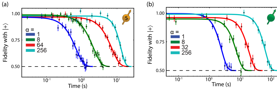
Figure 5.10: Dynamical decoupling of a single ^{13}\text{C} spin (C5) with \alpha = 1, 8, 64 and 256 pulses (a) and the ^{14}\text{N} spin with \alpha = 1, 8, 32 and 256 pulses (b). Each nuclear spin is initialised and read-out in the X-basis. We fit the data to the function f(t) = A + Be^{-(t/T)^n} (solid lines), where A = 0.5 , and B, T and n are fit parameters which account for the decay of the fidelity due to interactions with the nuclear spin bath, external noise and pulse errors. With 256 decoupling pulses, the fitted coherence times are T_2^{\alpha=256} = 12.9(4) s (C5, (a)) and T_2^{\alpha=256} = 63(2) s (14N, (b)).
