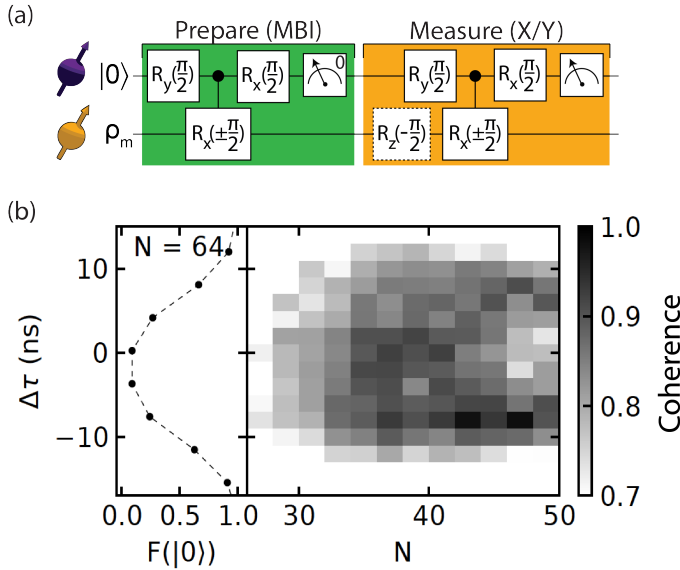
Figure 2.12: Two-qubit gate optimisation: (a) Quantum circuit used to initialise a single ^{13}\text{C} spin and measure the resulting expectation values \langle X \rangle and \langle Y \rangle . For the latter basis, the dashed R_z(-\pi/2) gate is incorporated. The '0' in the first electron measurement indicates that the sequences continues conditioned on receiving that outcome. (b) Measured coherence ( C = \sqrt{\langle X \rangle^2 + \langle Y \rangle^2} ) as a function of the number of decoupling pulses N and the adjustment of the interpulse delay from resonance, \Delta\tau . Combinations which produce the highest coherence correspond to the highest-fidelity two-qubit gates. Figure adapted from Kalb 59 .
