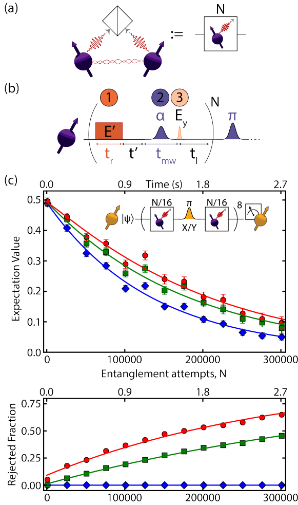
Figure 4.2: Memory robustness under remote-entanglement generation: (a) Sketch of a remote-entanglement process. After generation of local spin-photon entanglement at each node (see (b)), a detection event at a central beamsplitter heralds remote entanglement. Due to loss processes, the protocol is probabilistic. (b) Remote entanglement primitive: (1) The electron spin is reset by an optical pulse of duration t_r = 5 \mu\text{s} . (2) After a time t' = 200 \text{ ns} , a microwave pulse of duration t_{mw} = 2.8 \mu\text{s} prepares a spin superposition state. (3) An optical \pi -pulse generates spin-photon entanglement, after which a time t_l = 1 \mu\text{s} is required to determine whether the attempt succeeded. In case of success, a microwave \pi -pulse is used to preserve the electron coherence. E' and E_y denote optical transitions (Sec. 4.8). (c) Data qubit expectation value in the encoded state eigenbasis, as a function of the number of applied primitives (see (b)), averaged over the six cardinal states. Diamonds (squares and circles) correspond to no post-selection (post-selection on measuring \geq 1 and \geq 5 photons in a CR check performed at the end of the sequence). Solid lines are fits (see Sec. 4.8). Lower panel shows the fraction of rejected data for the three cases.
