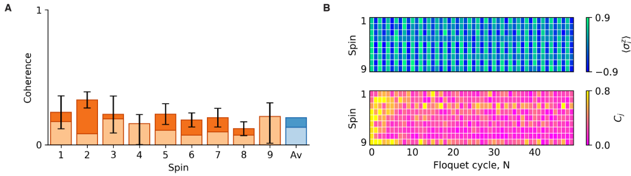
Figure 7.6: Individual spin data for Figs. 3E,G (A) Measured coherence for each spin after preparing the state |\uparrow\uparrow\uparrow\uparrow\uparrow\uparrow\uparrow\rangle (dark colored bars). The light shaded bars indicate the contribution from shot noise in the underlying measurements of \langle \sigma_j^x \rangle and \langle \sigma_j^y \rangle . The residual measured coherence is likely due to pulse errors in the \pi/2 basis rotations. The blue bar shows the average of the orange bars over all spins. The dark blue bar is used to indicate a baseline in Fig. 7.3G. (B) Individual spin magnetisations (top) and coherences (bottom) after preparing the superposition state [\cos(\pi/8)|\uparrow\rangle + \sin(\pi/8)|\downarrow\rangle]^{\otimes 9} .
