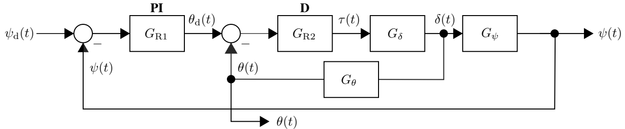
Figure 4. Nested control of steer \delta(t) and yaw \psi(t) .
