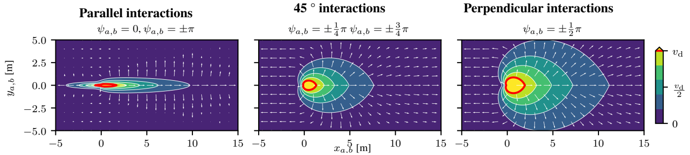
Figure 3. Repulsive force acting on a cyclist b interacting with a cyclist a (located at (0,0) , riding in x -direction) for different relative orientations \psi_{a,b} and positions (x_{a,b}, y_{a,b}) . Colors indicate the magnitude of the force field as multiples of the desired velocity v_d of b . At the red line, the repulsive force equals the maximum of b 's destination force. The force direction (black arrows) experienced by b is perpendicular to the contour lines. Parameter values: F_0 = 7 \frac{\text{m}}{\text{s}} , e_0 = 0.995 , e_1 = 0.7 , \sigma_0 = 0.5 \text{ m} , \sigma_1 = 5.0 \text{ m} , \sigma_2 = -0.3 \text{ m} , \sigma_3 = -4.9 \text{ m} .
