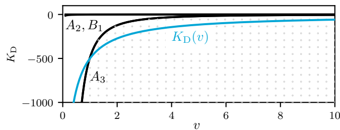
Figure 5. Stability limits (black lines) and stability region (gray dots) of the inner loop for K_D(v) with k_{d0} = -600 , k_{d1} = 0.2 , I_s = 0.07 \text{ kgm}^2 , c = 50 \text{ Nms} .
