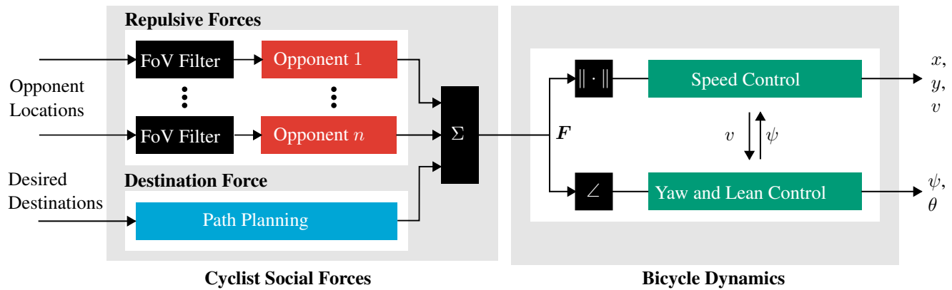
Figure 1. System overview of a cyclist with n opponents, experiencing the aggregated social forces F and controlling their speed v and yaw angle \psi accordingly. This also results in the bike's position x, y and roll angle \theta .
