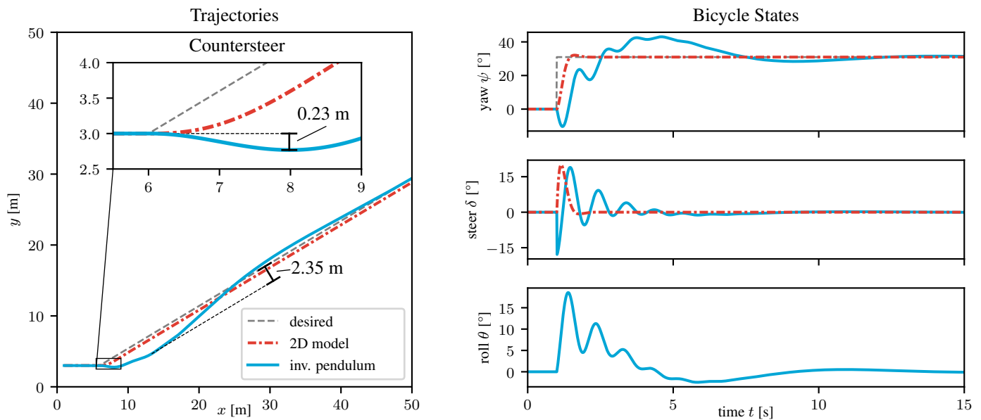
Figure 8. Yaw angle step response at constant speed. Comparison between the inverted pendulum bicycle dynamics (solid blue) and 2D bicycle dynamics (dash-dotted red). The left column shows the simulated trajectories with the reaction to a sudden change of the desired yaw angle. The right column shows the simulated bicycle states over time.
