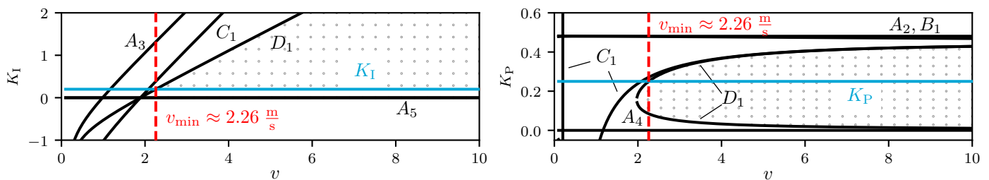
Figure 6. Stability limits (solid black) and stable area (gray dots) of the outer loop for the gains K_P = 0.25 and K_I = 0.2 . Capital letters naming the constraints refer to the corresponding coefficients of the Routh table.
