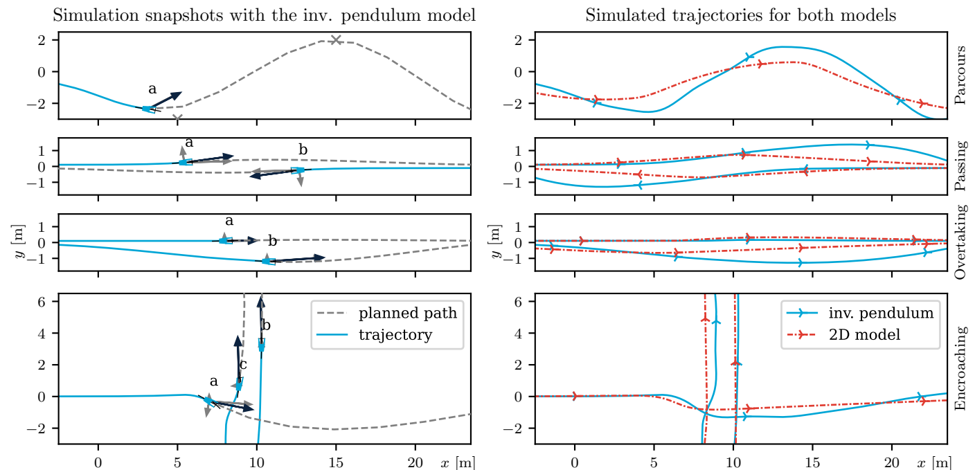
Figure 9. Simulations of interaction test scenarios (top to bottom: 'parcours', 'passing', 'overtaking', 'encroaching'). The left shows simulation snapshots of inverted pendulum bikes during interaction. Arrows indicate the individual social forces experienced by the cyclist (gray) and the resulting force (dark blue). The right compares the simulated trajectories of inverted pendulum bikes (solid blue) and 2D bikes (dash-dotted red).
