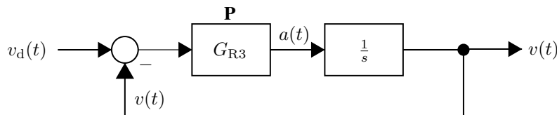
Figure 7. Speed control.
