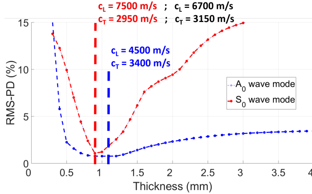
Figure 4.10: Minimum RMS-PD error of measured error maps for an aluminum pipe as a function of thickness h for the A_0 mode (blue) and the mode S_0 (red). The values of longitudinal and shear wave speeds are expressed for thicknesses with lowest error ( h = 0.9 mm for the S_0 wave mode, h = 1.1 mm for the A_0 wave mode). The wave speeds obtained by fitting the A_0 mode with a plate of thickness h = 0.9 mm are reported in black.
