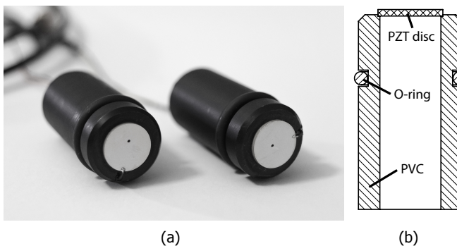
Figure 5.4: Pair of transducers made of an air-backed piezo-ceramic disc mounted onto a PVC cylinder.
