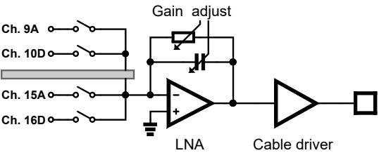
Figure 2.24: Block diagram of the LNA.
