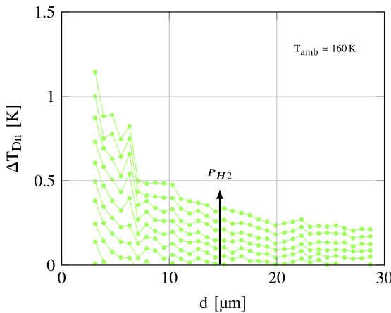
FIGURE 13. Substrate heating measured by the 'dense' array ( \Delta T_{Dn} ) as a function of distance to the center heater ( d ) at different heater power levels: P_{H2} = \{0.6, 1.2, 1.7, 2.3, 3.0, 3.6, 4.3, 5.0, 5.8, 6.6\} mW. T_{amb} = 160 K. Only curves corresponding to P_{H2} values causing significant heating are plotted. T_{amb} was selected for clearly showing the effects of T_{drift} , similar curves were found at other T_{amb} .
