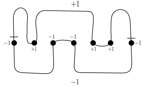
Fig. 4. A schematic proof why the hypothesis set H_c has an infinite VC-dimension. The embedded circle, its upper half assigning points to +1 and its lower half to -1, can label the seven points correctly.
