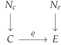
Fig. 2. Simple functional causal model [16]. The effect E is caused by C given a deterministic mapping \rho . E and C are influenced by noise variables N_E and N_C , respectively.
