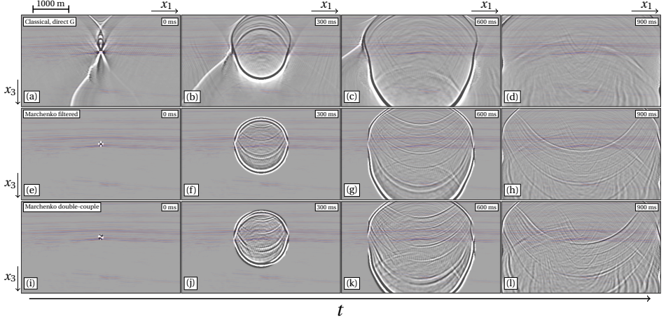
Figure 2.9: Snapshots of the homogeneous Green's function in the subsurface of the Vøring basin, obtained using the classical representation of Equation (2.9) for a monopole source at (a) 0ms, (b) 300ms, (c) 600ms and (d) 900ms. Idem, using the single-sided representation of Equation (2.10) for a monopole source at (e) 0ms, (f) 300ms, (g) 600ms and (h) 900ms. Idem, using the single-sided representation of Equation (2.15) for a double-couple source inclined at -20 degrees at (i) 0ms, (j) 300ms, (k) 600ms and (l) 900ms. All data contain a 30Hz Ricker wavelet.
