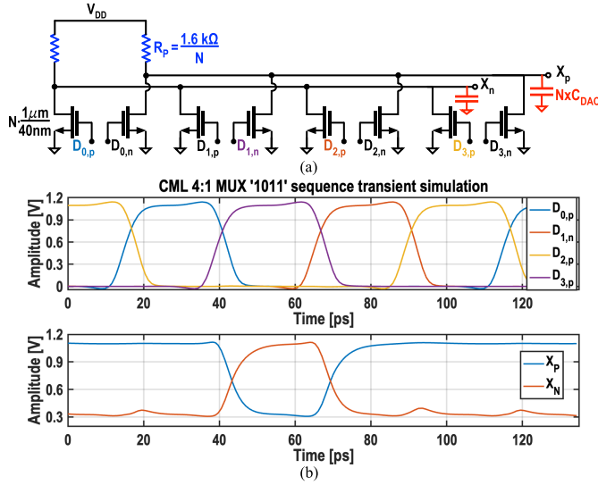
Fig. 10. (a) Schematic of the 4:1 CML MUX. The pull-up resistors ( R_p ) are inversely proportional to the size of their corresponding DAC slice with an input parasitic capacitance of N \times C_{DAC} . (b) Simulated input and output waveforms of the 4:1 CML MUX for a “1011” sequence.
