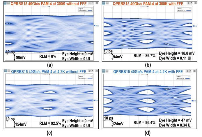
Fig. 22. Measured 40-Gb/s PAM4 eye diagrams with 1.2-m channel—(a) without FFE at 300 K, (b) with FFE at 300 K, (c) without FFE at 4.2 K, and (d) with FFE at 4.2 K.
