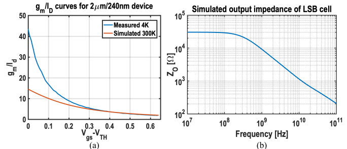
Fig. 8. (a) RT simulation and CT measurement of g_m/I_D curves for a 2- \mu\text{m}/240\text{-nm} transistor. (b) Simulated output impedance of the DAC LSB cell versus frequency.
