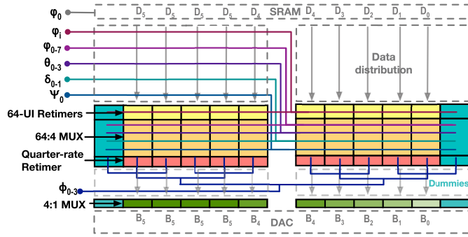
Fig. 15. Illustration of the clock distribution layout. The data distribution is done vertically, indicated in gray; the clock lines are distributed horizontally indicated with the different colors.
