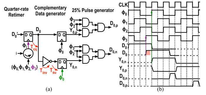
Fig. 11. Quarter-rate retimer, complementary data generator, and 25% pulse generator. (a) Schematic illustrating the worst case critical path in red. (b) Timing diagram showing the total delay.
