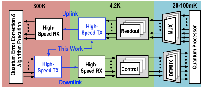
Fig. 1. Simplified block diagram of a scalable quantum computing system incorporating a cryo-CMOS high-speed wireline link.
