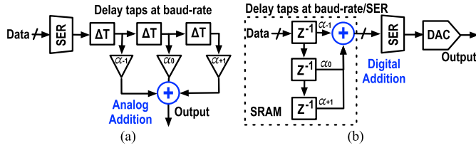
Fig. 5. FFE implementation in (a) analog domain and (b) digital domain.
