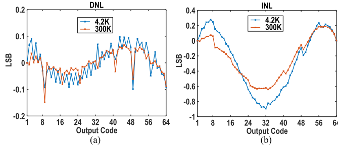
Fig. 19. Measured (a) DNL and (b) INL at 4.2 and 300 K.
